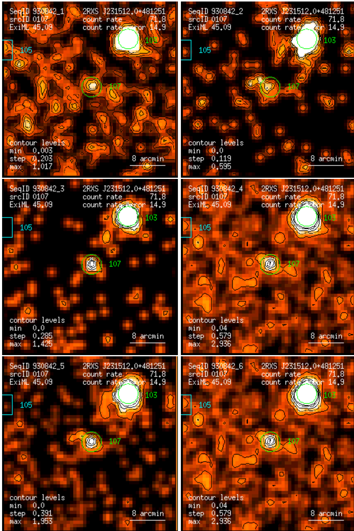
Figure 107: RASS 930842: detection 0107: band rate images, Gaussian filter: (1) PSPC channels 11 – 41, (2) 52 – 90, (3) 91 – 201, (4) 11 – 235, (5) 52 – 201, (6) 11 – 201. Broad band rates in counts/ks. Band rate contour levels in counts/ks/arcmin 2 .
