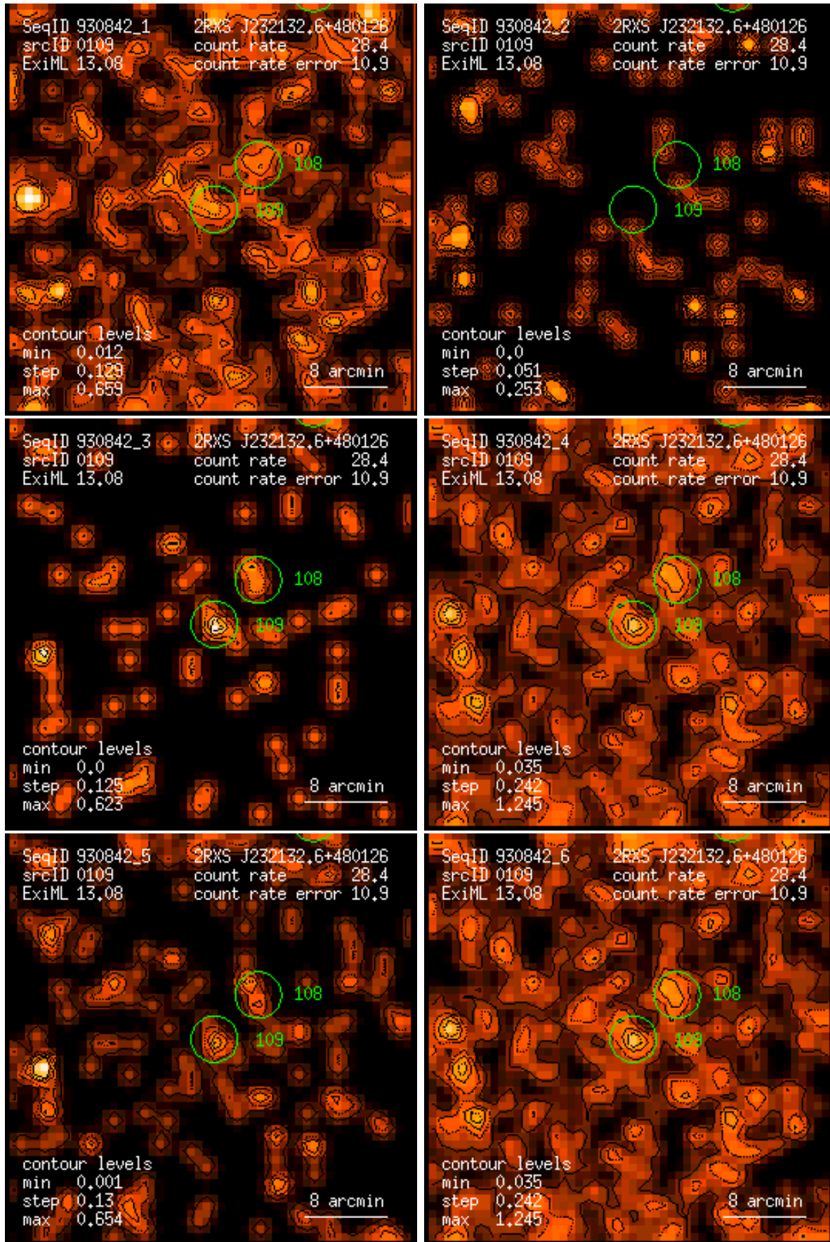
Figure 109: RASS 930842: detection 0109: band rate images, Gaussian filter: (1) PSPC channels 11 – 41, (2) 52 – 90, (3) 91 – 201, (4) 11 – 235, (5) 52 – 201, (6) 11 – 201. Broad band rates in counts/ks. Band rate contour levels in counts/ks/arcmin 2 .
