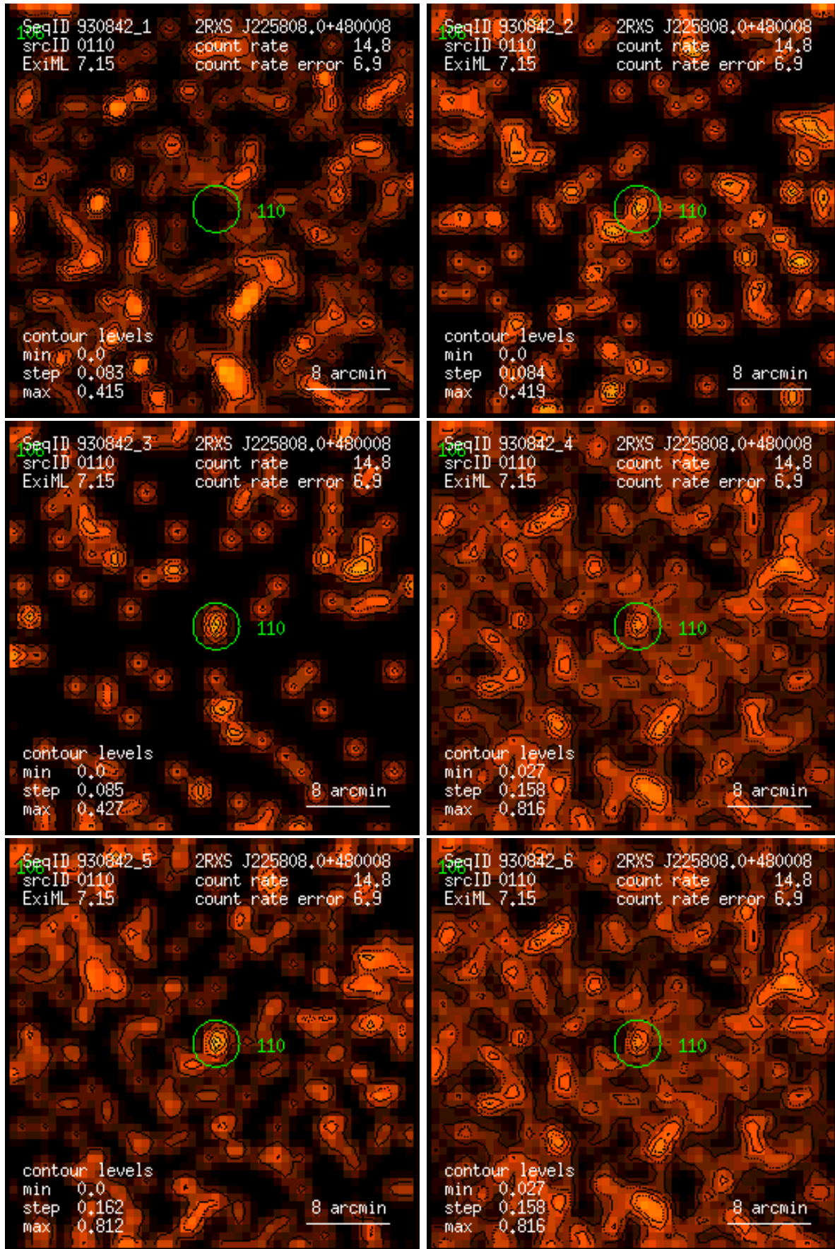
Figure 110: RASS 930842: detection 0110: band rate images, Gaussian filter: (1) PSPC channels 11 – 41, (2) 52 – 90, (3) 91 – 201, (4) 11 – 235, (5) 52 – 201, (6) 11 – 201. Broad band rates in counts/ks. Band rate contour levels in counts/ks/arcmin 2 .
