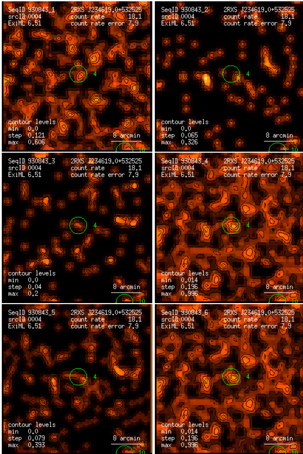
Figure 4: RASS 930843: detection 0004: band rate images, Gaussian filter: (1) PSPC channels 11 – 41, (2) 52 – 90, (3) 91 – 201, (4) 11 – 235, (5) 52 – 201, (6) 11 – 201. Broad band rates in counts/ks. Band rate contour levels in counts/ks/arcmin 2 .
