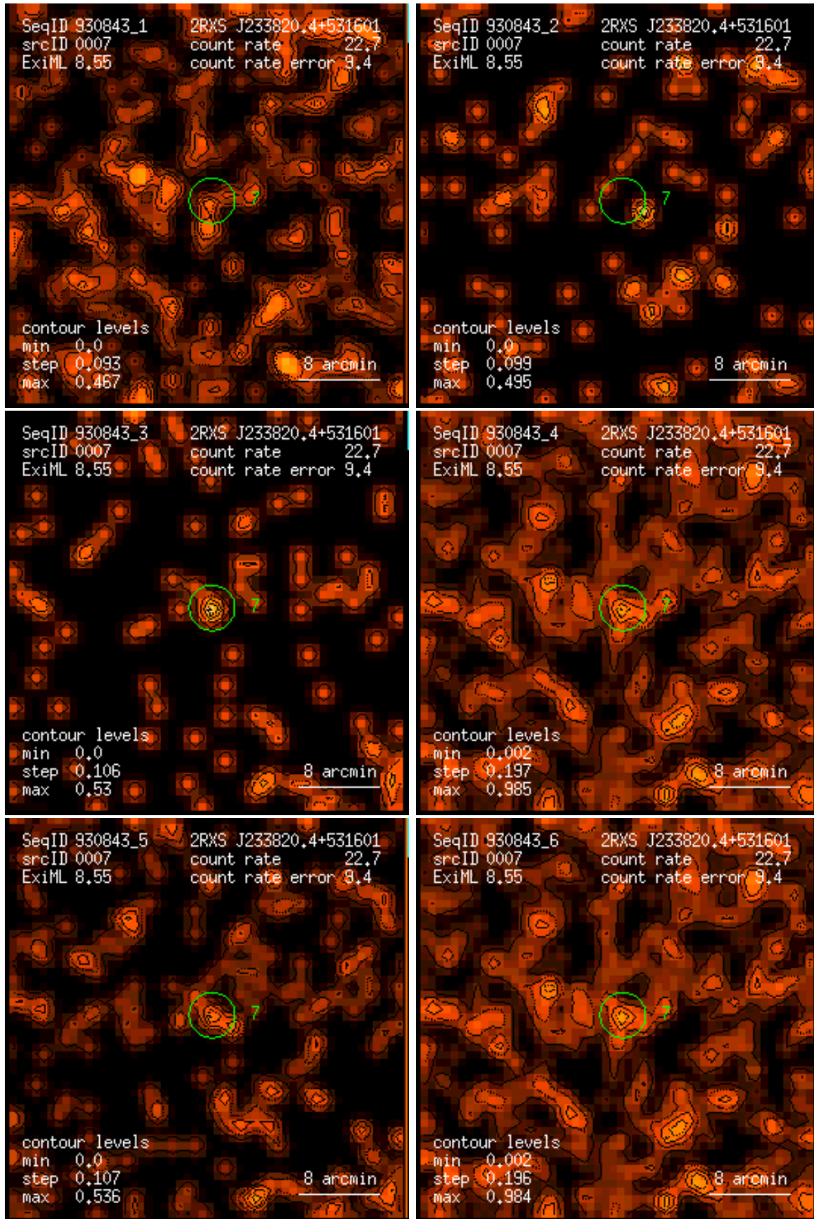
Figure 7: RASS 930843: detection 0007: band rate images, Gaussian filter: (1) PSPC channels 11 – 41, (2) 52 – 90, (3) 91 – 201, (4) 11 – 235, (5) 52 – 201, (6) 11 – 201. Broad band rates in counts/ks. Band rate contour levels in counts/ks/arcmin 2 .
