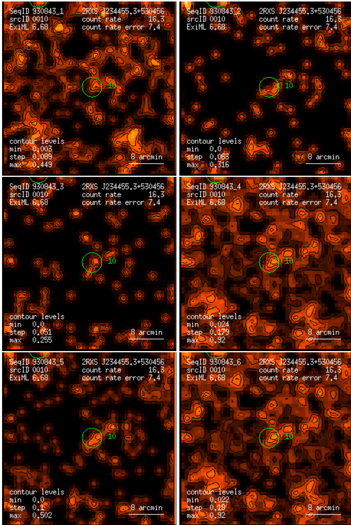
Figure 10: RASS 930843: detection 0010: band rate images, Gaussian filter: (1) PSPC channels 11 – 41, (2) 52 – 90, (3) 91 – 201, (4) 11 – 235, (5) 52 – 201, (6) 11 – 201. Broad band rates in counts/ks. Band rate contour levels in counts/ks/arcmin 2 .
