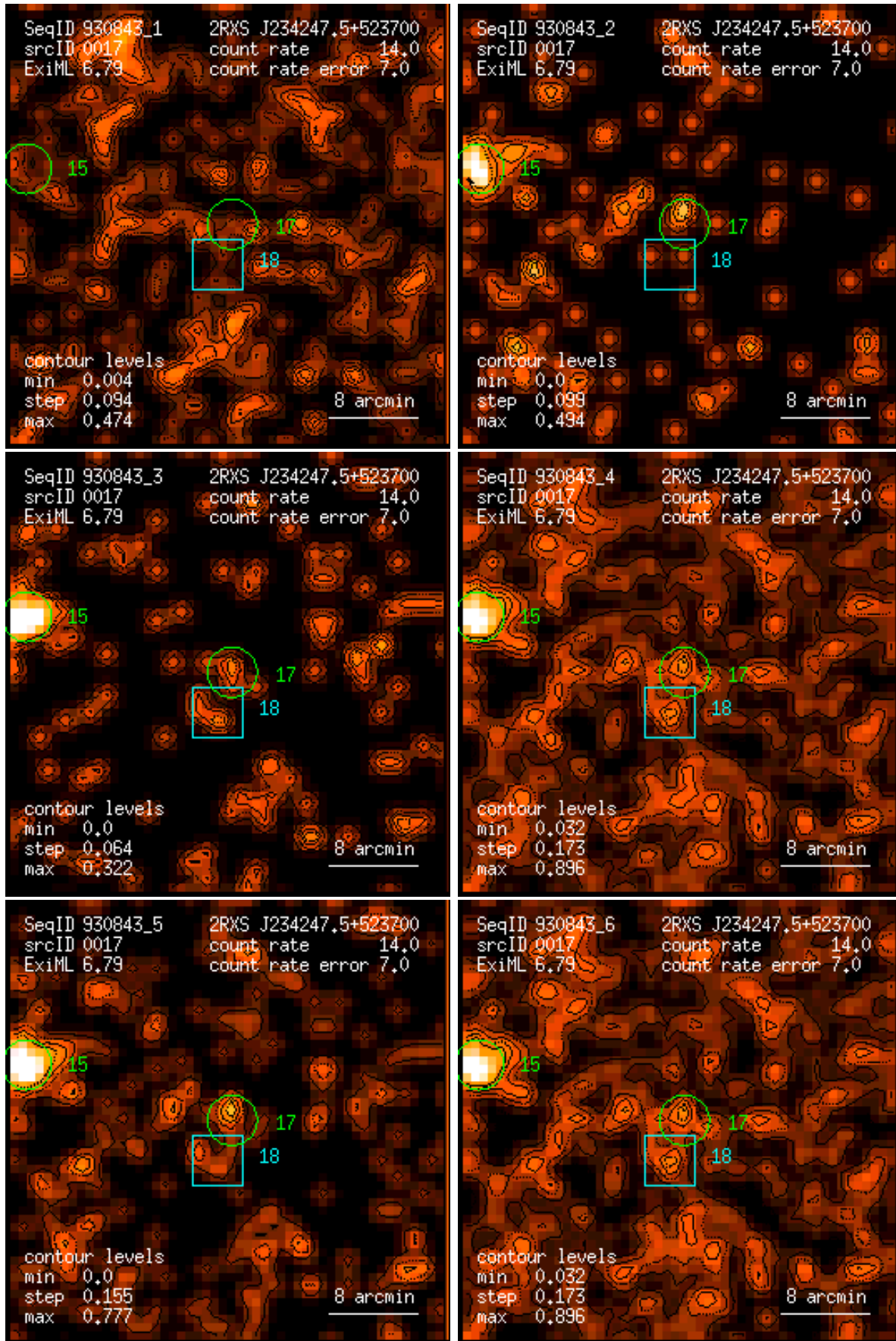
Figure 17: RASS 930843: detection 0017: band rate images, Gaussian filter: (1) PSPC channels 11 – 41, (2) 52 – 90, (3) 91 – 201, (4) 11 – 235, (5) 52 – 201, (6) 11 – 201. Broad band rates in counts/ks. Band rate contour levels in counts/ks/arcmin 2 .
