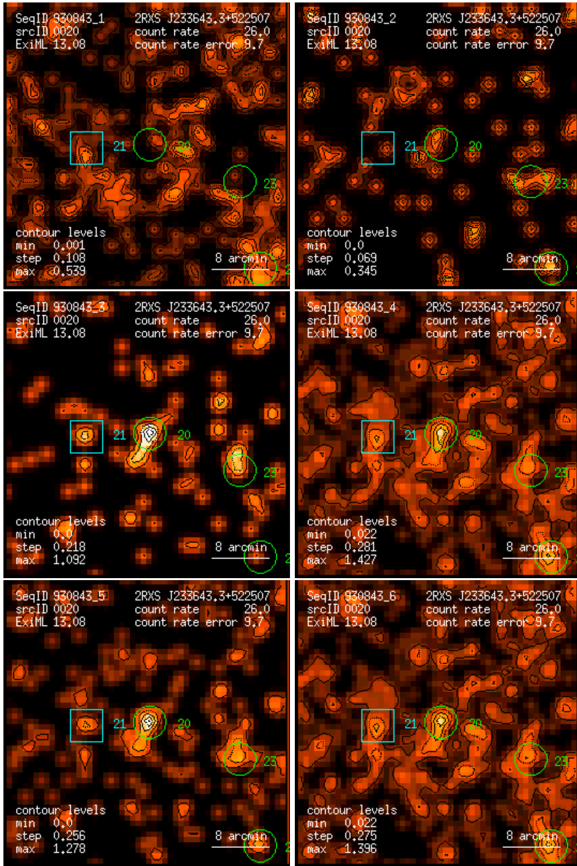
Figure 20: RASS 930843: detection 0020: band rate images, Gaussian filter: (1) PSPC channels 11 – 41, (2) 52 – 90, (3) 91 – 201, (4) 11 – 235, (5) 52 – 201, (6) 11 – 201. Broad band rates in counts/ks. Band rate contour levels in counts/ks/arcmin 2 .
