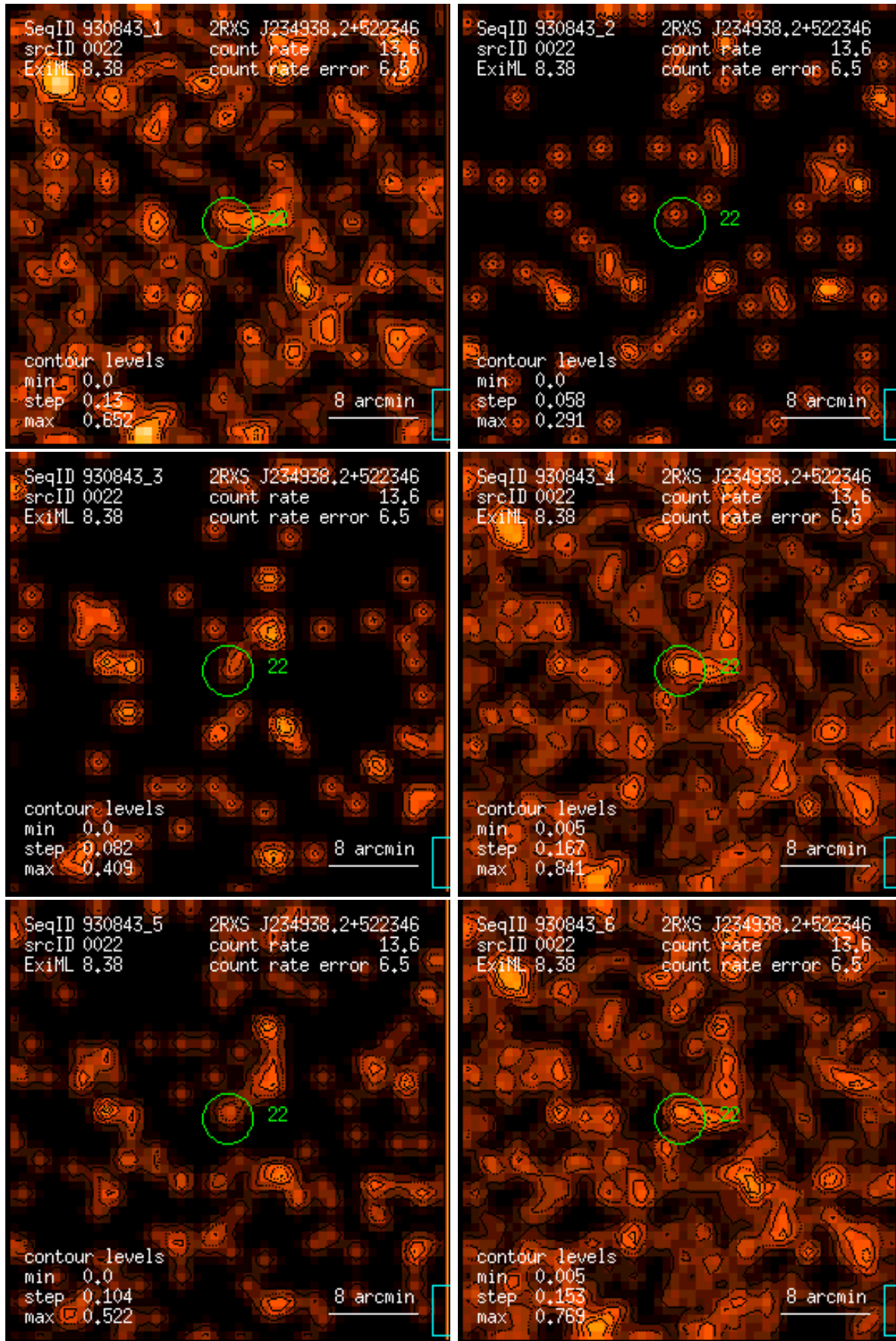
Figure 22: RASS 930843: detection 0022: band rate images, Gaussian filter: (1) PSPC channels 11 – 41, (2) 52 – 90, (3) 91 – 201, (4) 11 – 235, (5) 52 – 201, (6) 11 – 201. Broad band rates in counts/ks. Band rate contour levels in counts/ks/arcmin 2 .
