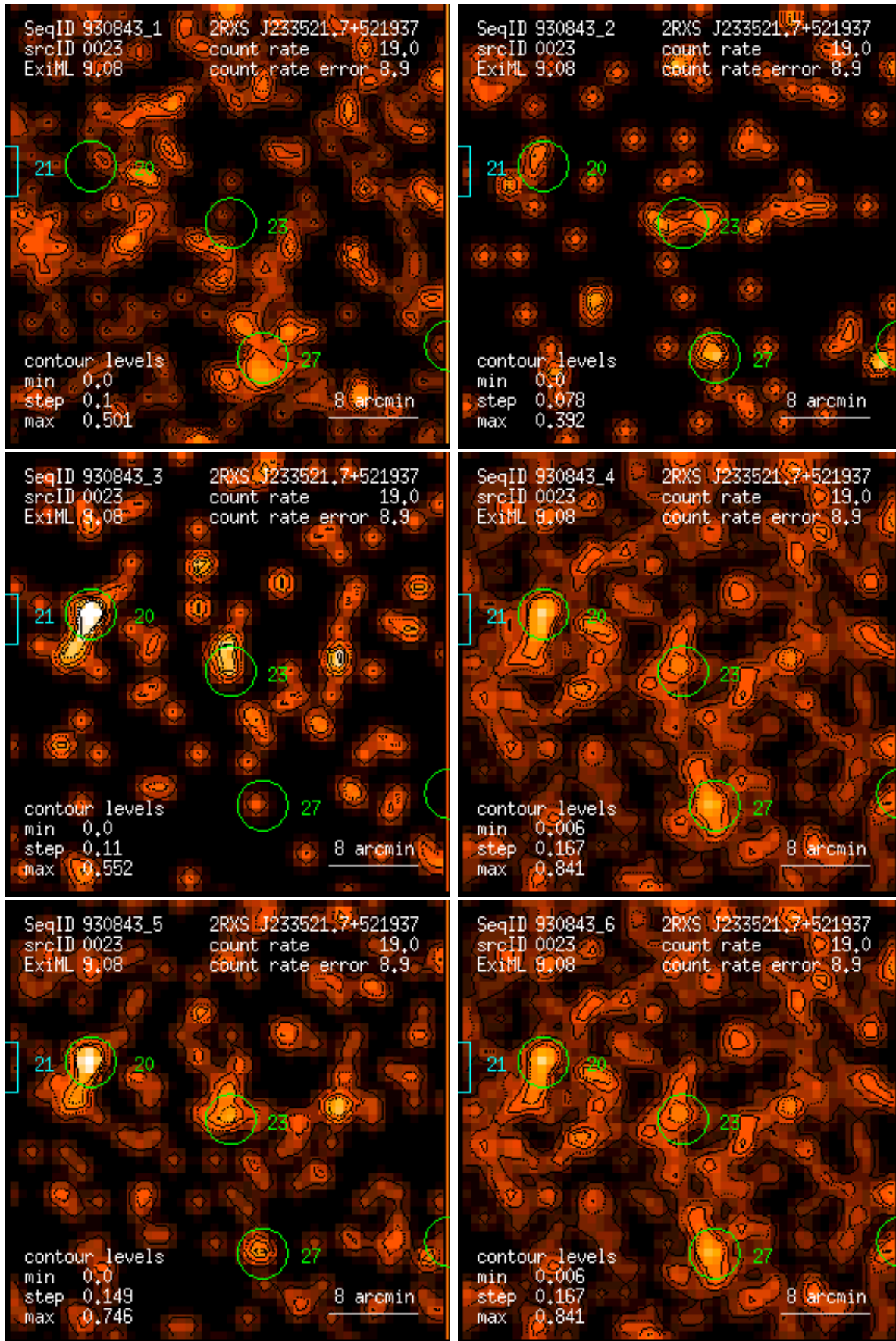
Figure 23: RASS 930843: detection 0023: band rate images, Gaussian filter: (1) PSPC channels 11 – 41, (2) 52 – 90, (3) 91 – 201, (4) 11 – 235, (5) 52 – 201, (6) 11 – 201. Broad band rates in counts/ks. Band rate contour levels in counts/ks/arcmin 2 .
