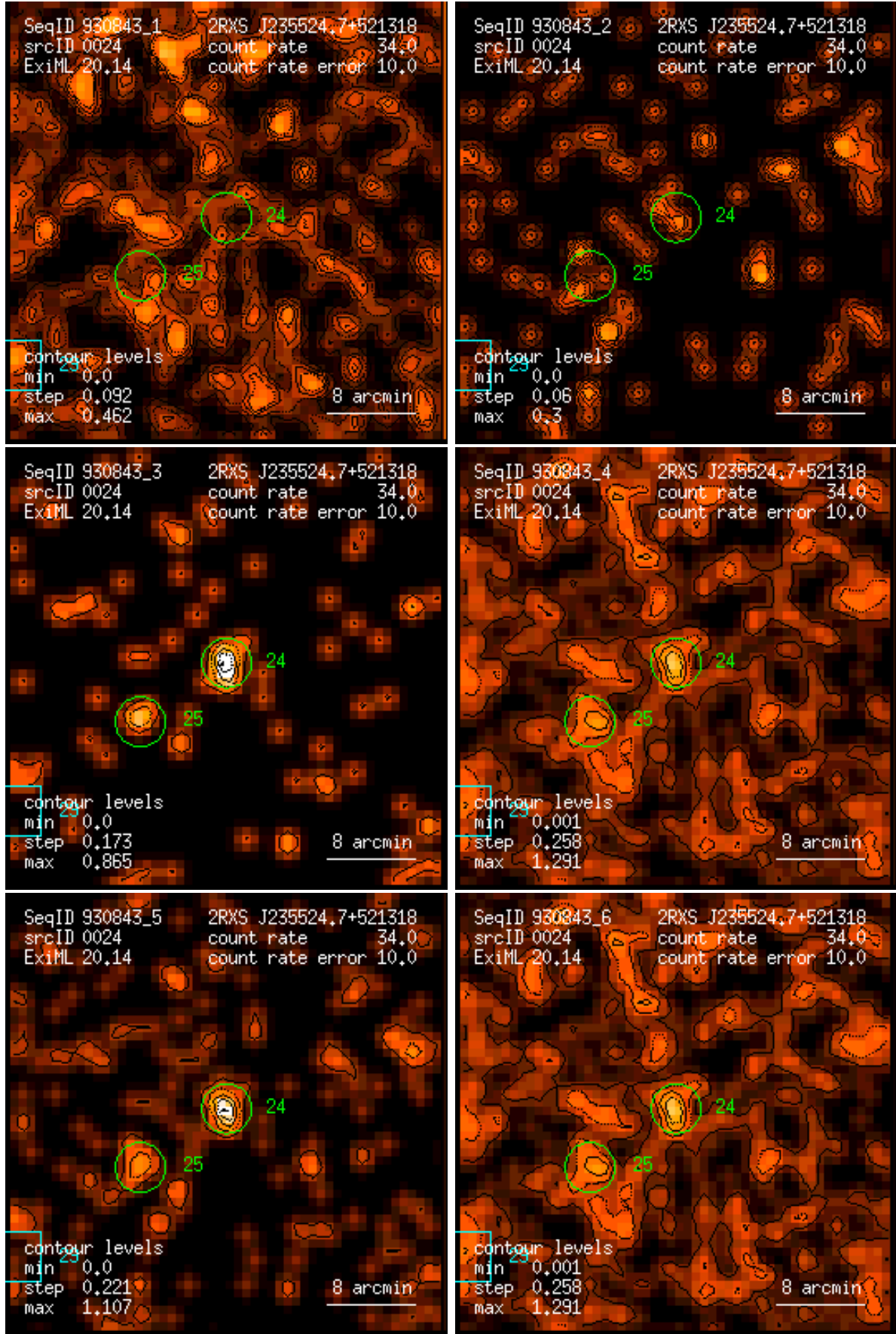
Figure 24: RASS 930843: detection 0024: band rate images, Gaussian filter: (1) PSPC channels 11 – 41, (2) 52 – 90, (3) 91 – 201, (4) 11 – 235, (5) 52 – 201, (6) 11 – 201. Broad band rates in counts/ks. Band rate contour levels in counts/ks/arcmin 2 .
