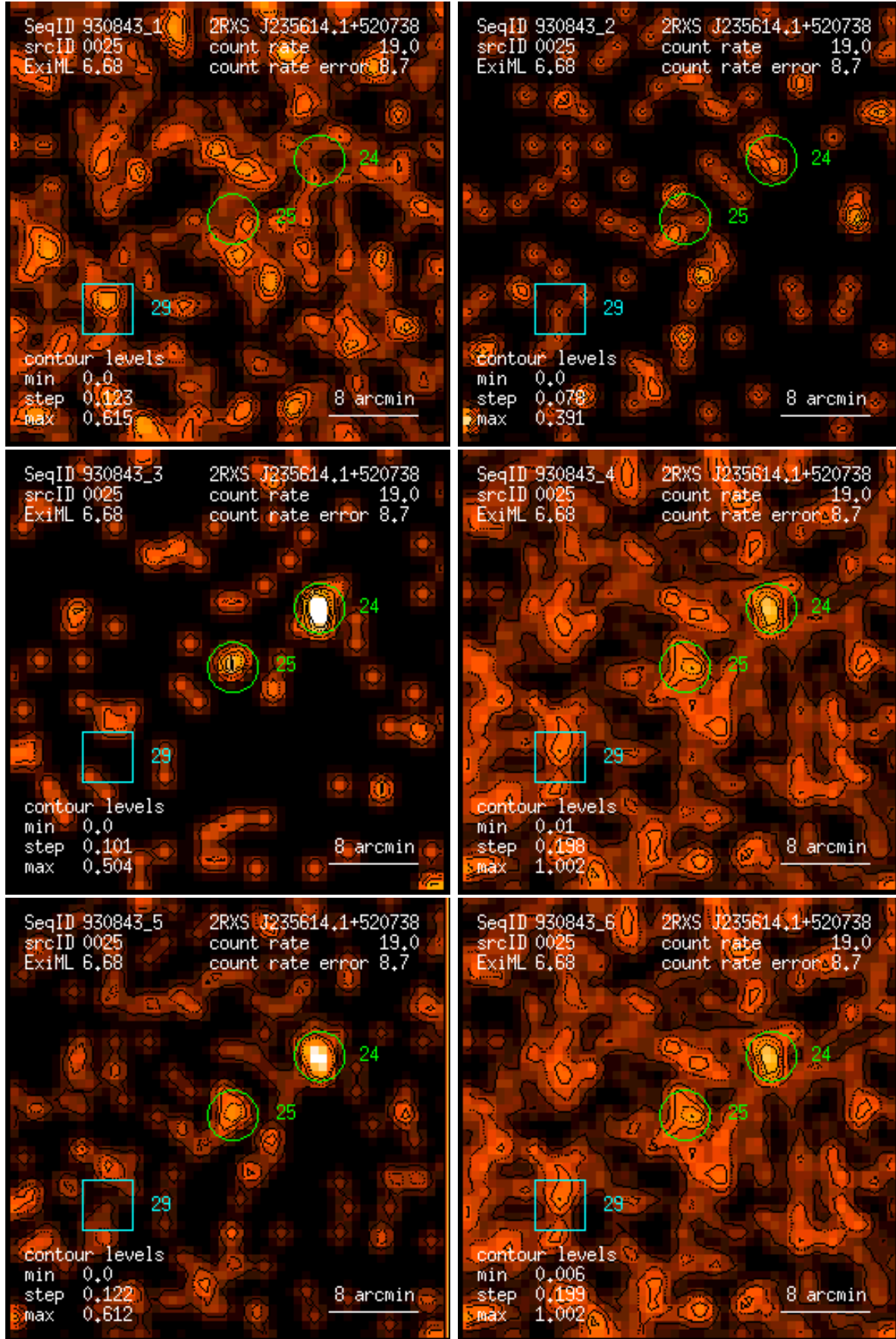
Figure 25: RASS 930843: detection 0025: band rate images, Gaussian filter: (1) PSPC channels 11 – 41, (2) 52 – 90, (3) 91 – 201, (4) 11 – 235, (5) 52 – 201, (6) 11 – 201. Broad band rates in counts/ks. Band rate contour levels in counts/ks/arcmin 2 .
