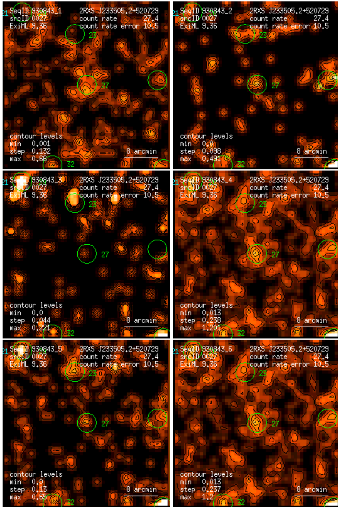
Figure 27: RASS 930843: detection 0027: band rate images, Gaussian filter: (1) PSPC channels 11 – 41, (2) 52 – 90, (3) 91 – 201, (4) 11 – 235, (5) 52 – 201, (6) 11 – 201. Broad band rates in counts/ks. Band rate contour levels in counts/ks/arcmin 2 .
