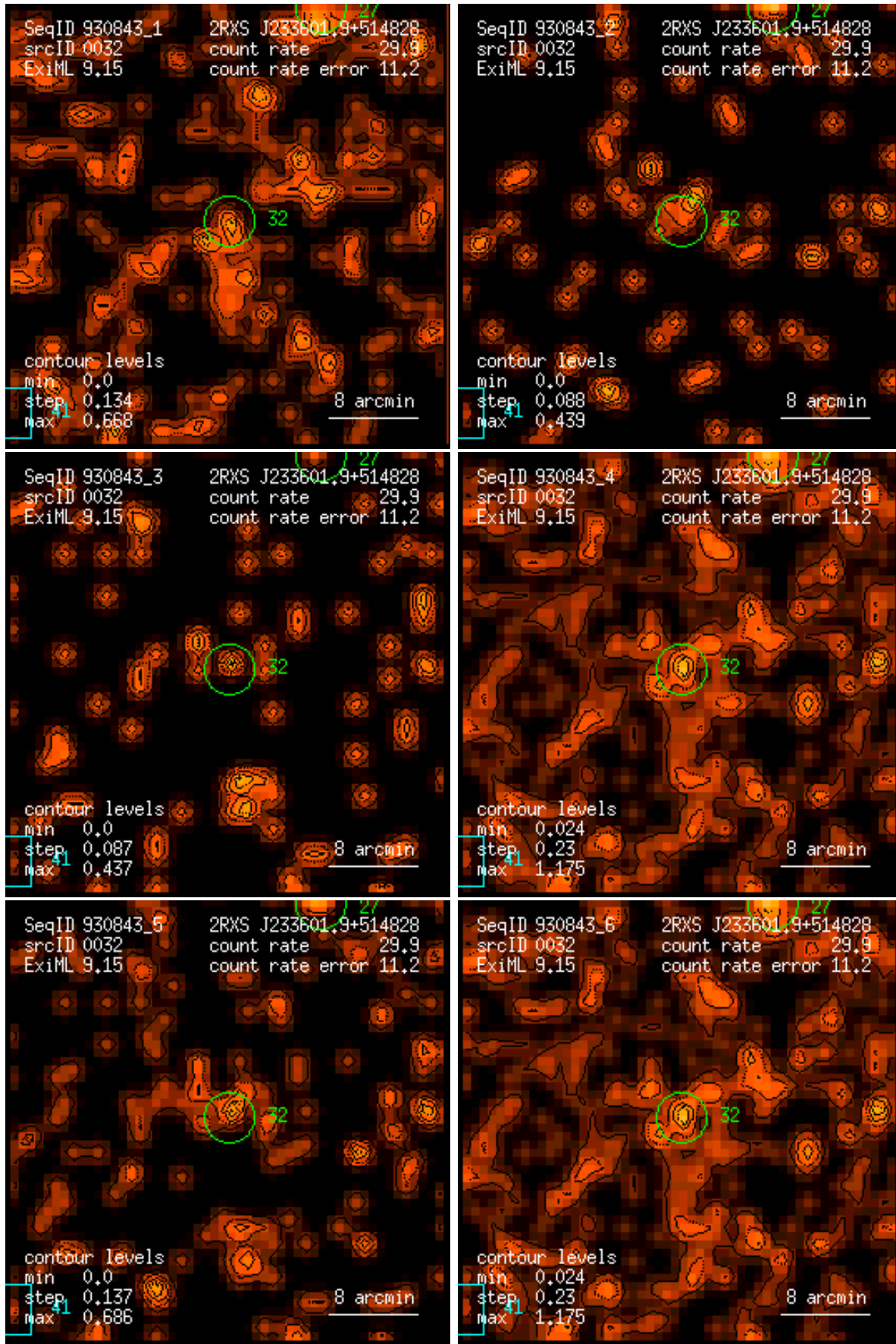
Figure 32: RASS 930843: detection 0032: band rate images, Gaussian filter: (1) PSPC channels 11 – 41, (2) 52 – 90, (3) 91 – 201, (4) 11 – 235, (5) 52 – 201, (6) 11 – 201. Broad band rates in counts/ks. Band rate contour levels in counts/ks/arcmin 2 .
