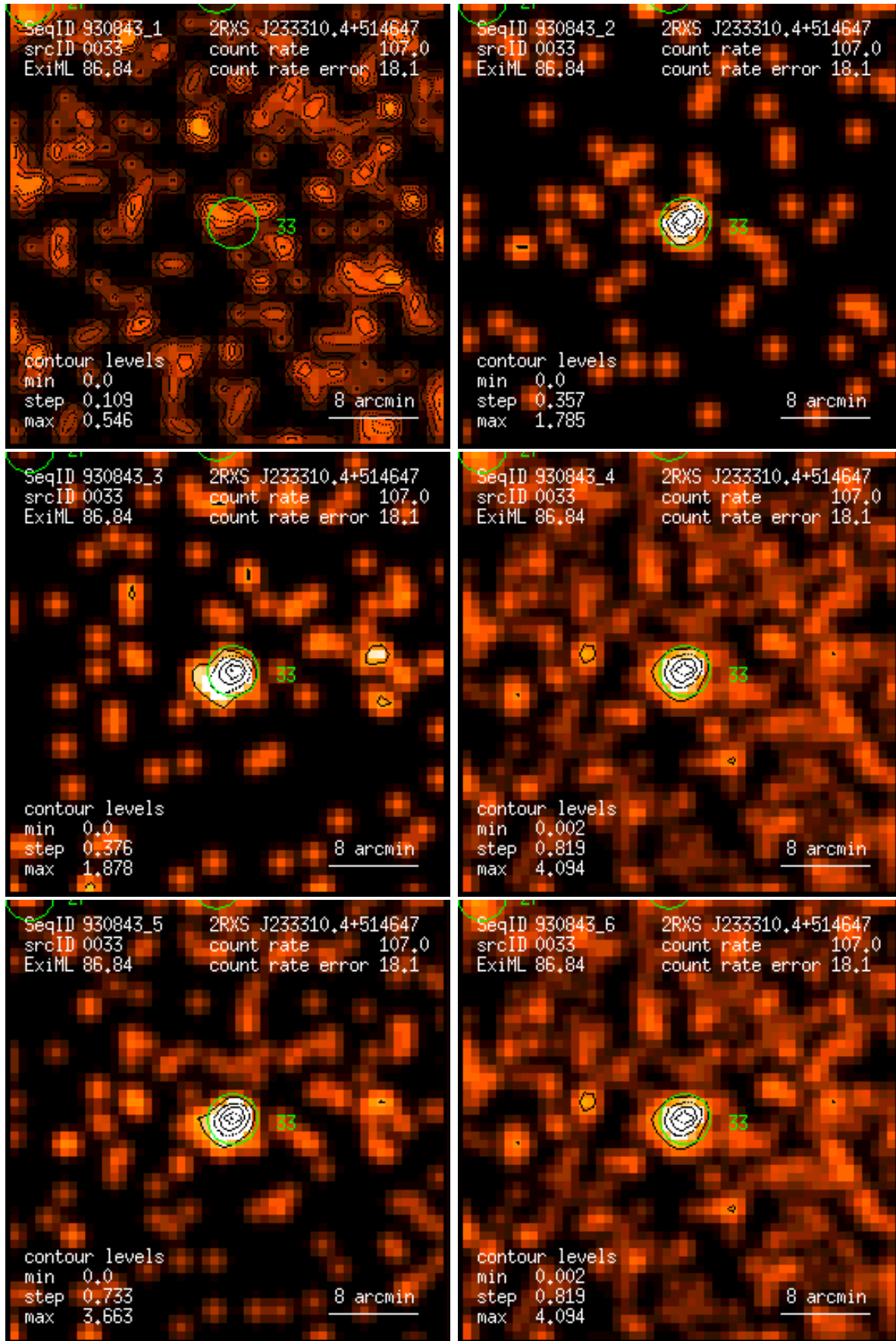
Figure 33: RASS 930843: detection 0033: band rate images, Gaussian filter: (1) PSPC channels 11 – 41, (2) 52 – 90, (3) 91 – 201, (4) 11 – 235, (5) 52 – 201, (6) 11 – 201. Broad band rates in counts/ks. Band rate contour levels in counts/ks/arcmin 2 .
