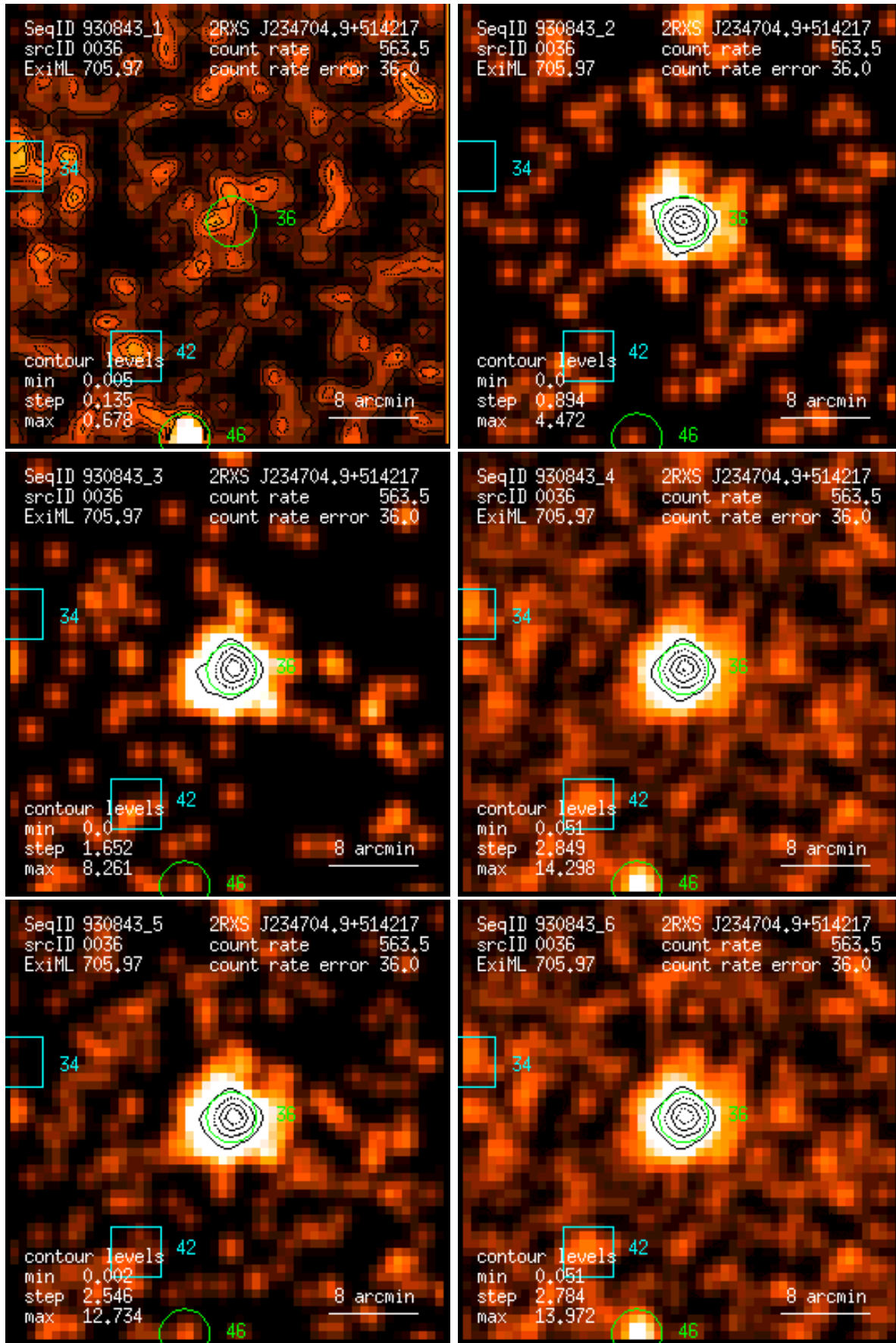
Figure 36: RASS 930843: detection 0036: band rate images, Gaussian filter: (1) PSPC channels 11 – 41, (2) 52 – 90, (3) 91 – 201, (4) 11 – 235, (5) 52 – 201, (6) 11 – 201. Broad band rates in counts/ks. Band rate contour levels in counts/ks/arcmin 2 .
