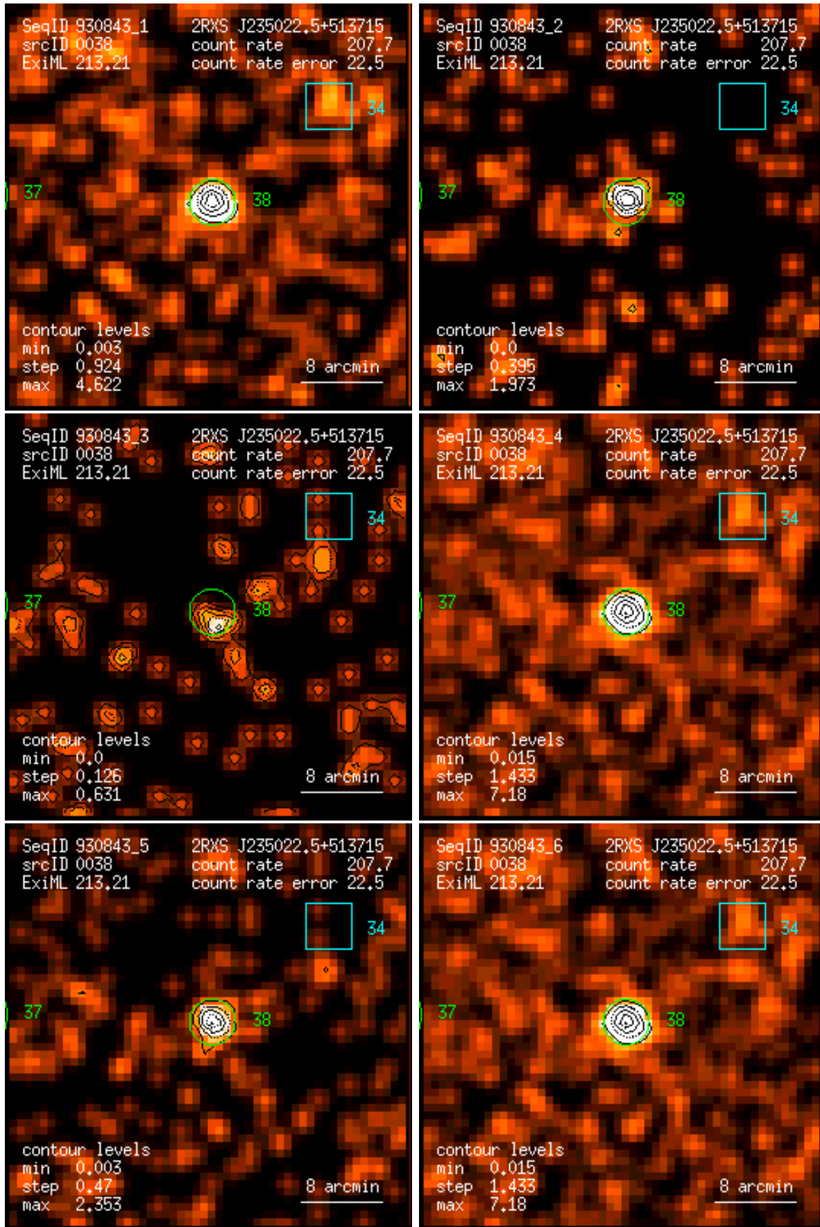
Figure 38: RASS 930843: detection 0038: band rate images, Gaussian filter: (1) PSPC channels 11 – 41, (2) 52 – 90, (3) 91 – 201, (4) 11 – 235, (5) 52 – 201, (6) 11 – 201. Broad band rates in counts/ks. Band rate contour levels in counts/ks/arcmin 2 .
