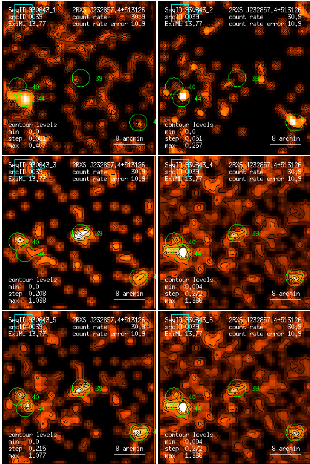
Figure 39: RASS 930843: detection 0039: band rate images, Gaussian filter: (1) PSPC channels 11 – 41, (2) 52 – 90, (3) 91 – 201, (4) 11 – 235, (5) 52 – 201, (6) 11 – 201. Broad band rates in counts/ks. Band rate contour levels in counts/ks/arcmin 2 .
