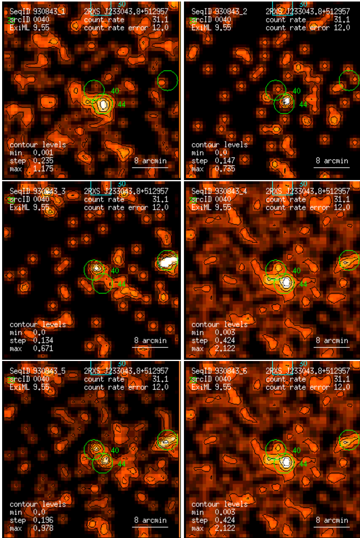
Figure 40: RASS 930843: detection 0040: band rate images, Gaussian filter: (1) PSPC channels 11 – 41, (2) 52 – 90, (3) 91 – 201, (4) 11 – 235, (5) 52 – 201, (6) 11 – 201. Broad band rates in counts/ks. Band rate contour levels in counts/ks/arcmin 2 .
