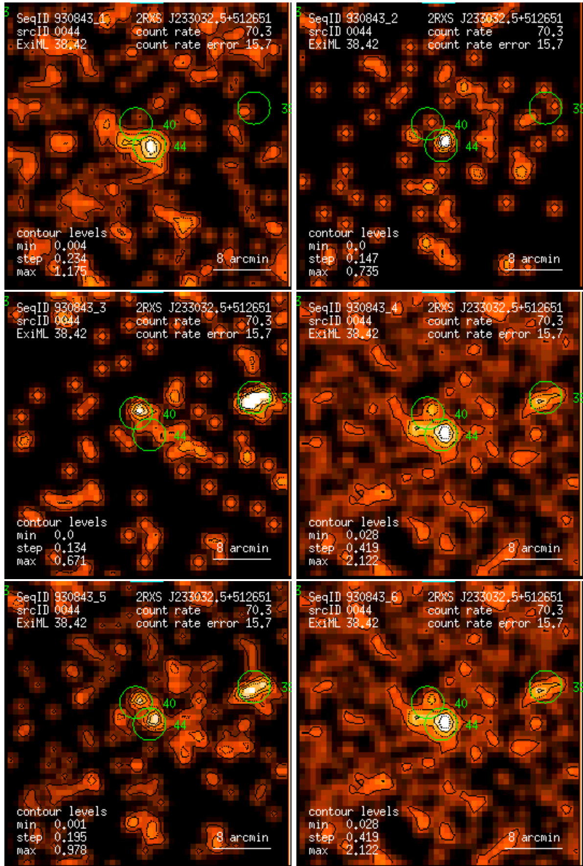
Figure 44: RASS 930843: detection 0044: band rate images, Gaussian filter: (1) PSPC channels 11 – 41, (2) 52 – 90, (3) 91 – 201, (4) 11 – 235, (5) 52 – 201, (6) 11 – 201. Broad band rates in counts/ks. Band rate contour levels in counts/ks/arcmin 2 .
