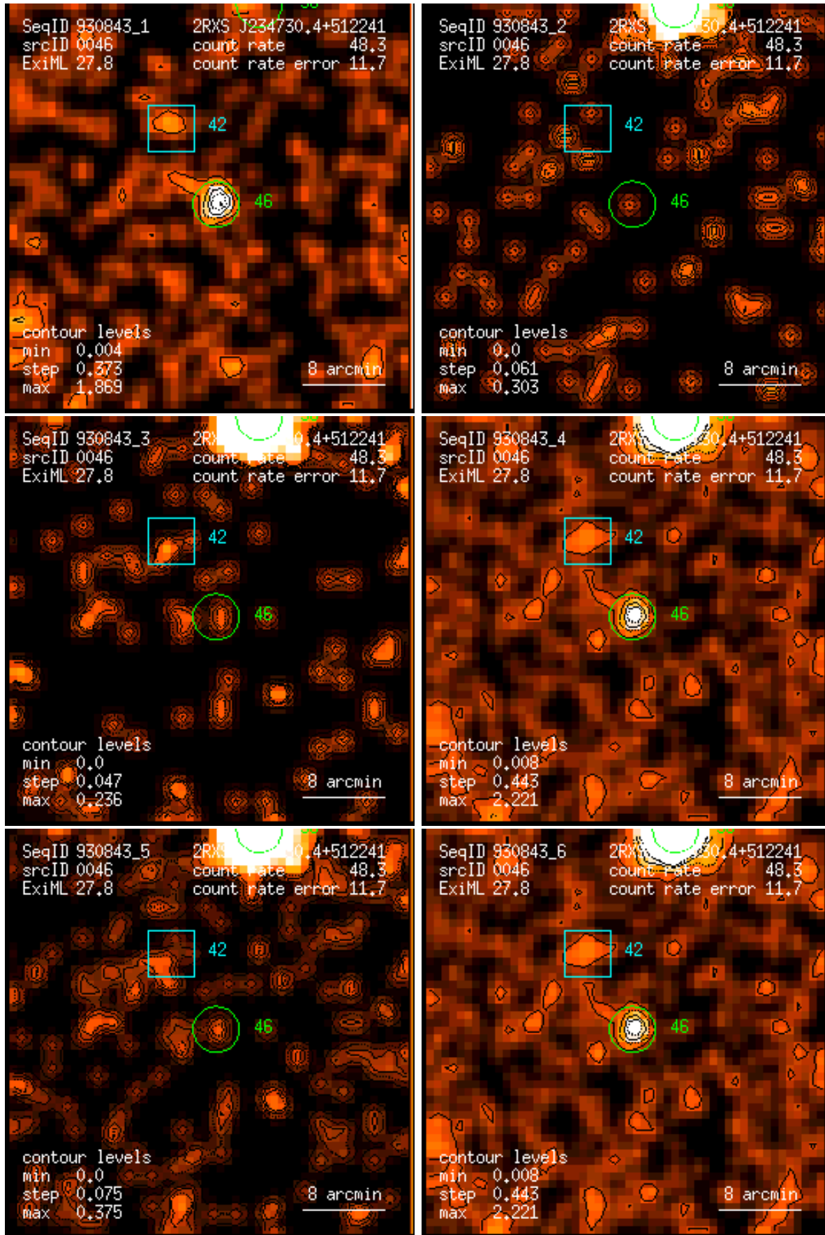
Figure 46: RASS 930843: detection 0046: band rate images, Gaussian filter: (1) PSPC channels 11 – 41, (2) 52 – 90, (3) 91 – 201, (4) 11 – 235, (5) 52 – 201, (6) 11 – 201. Broad band rates in counts/ks. Band rate contour levels in counts/ks/arcmin 2 .
