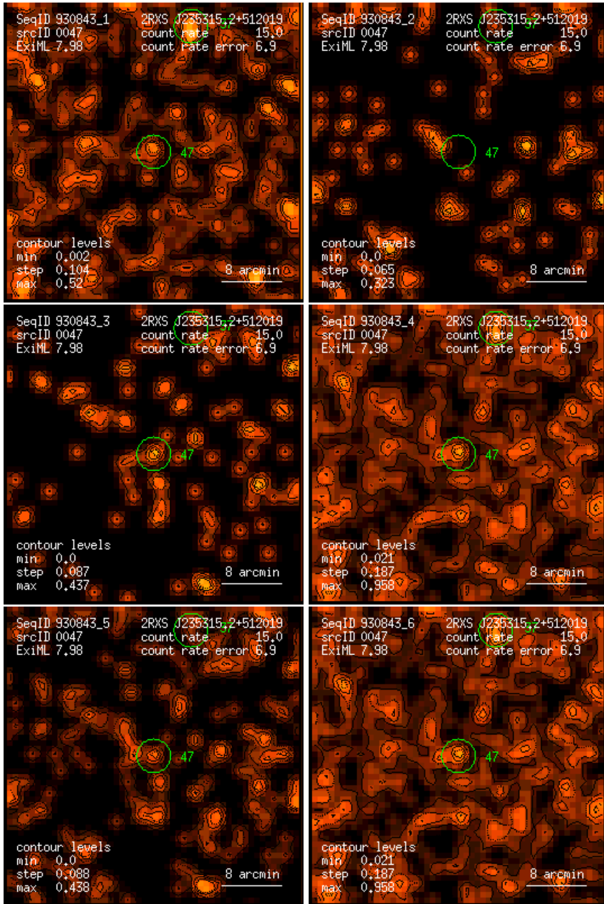
Figure 47: RASS 930843: detection 0047: band rate images, Gaussian filter: (1) PSPC channels 11 – 41, (2) 52 – 90, (3) 91 – 201, (4) 11 – 235, (5) 52 – 201, (6) 11 – 201. Broad band rates in counts/ks. Band rate contour levels in counts/ks/arcmin 2 .
