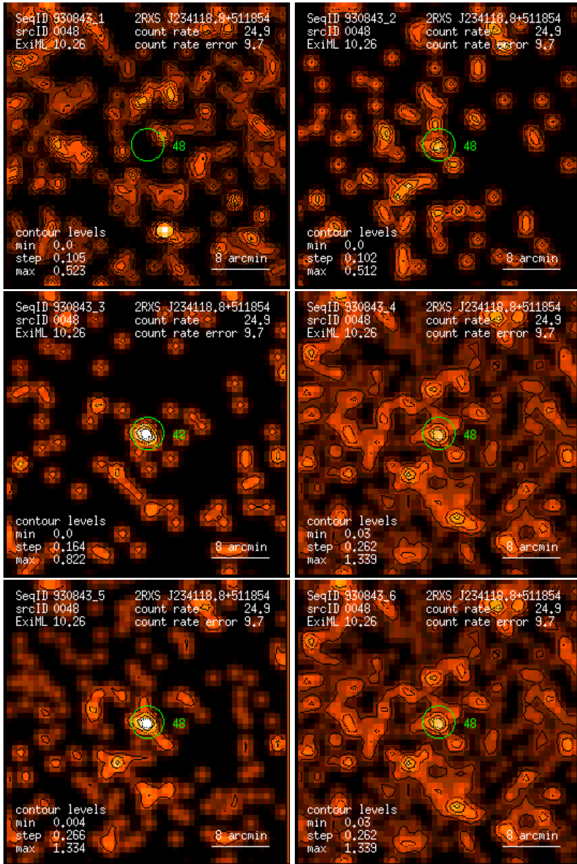
Figure 48: RASS 930843: detection 0048: band rate images, Gaussian filter: (1) PSPC channels 11 – 41, (2) 52 – 90, (3) 91 – 201, (4) 11 – 235, (5) 52 – 201, (6) 11 – 201. Broad band rates in counts/ks. Band rate contour levels in counts/ks/arcmin 2 .
