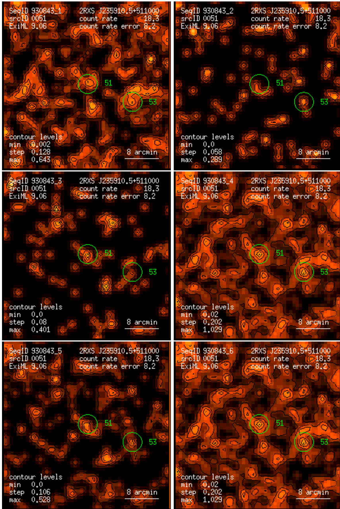
Figure 51: RASS 930843: detection 0051: band rate images, Gaussian filter: (1) PSPC channels 11 – 41, (2) 52 – 90, (3) 91 – 201, (4) 11 – 235, (5) 52 – 201, (6) 11 – 201. Broad band rates in counts/ks. Band rate contour levels in counts/ks/arcmin 2 .
