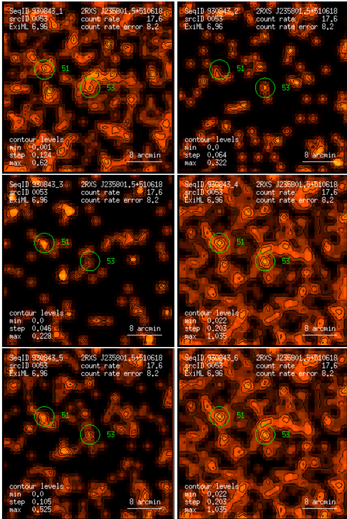
Figure 53: RASS 930843: detection 0053: band rate images, Gaussian filter: (1) PSPC channels 11 – 41, (2) 52 – 90, (3) 91 – 201, (4) 11 – 235, (5) 52 – 201, (6) 11 – 201. Broad band rates in counts/ks. Band rate contour levels in counts/ks/arcmin 2 .
