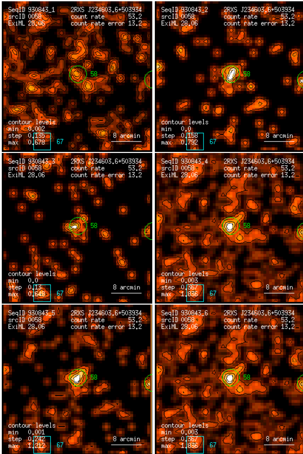
Figure 58: RASS 930843: detection 0058: band rate images, Gaussian filter: (1) PSPC channels 11 – 41, (2) 52 – 90, (3) 91 – 201, (4) 11 – 235, (5) 52 – 201, (6) 11 – 201. Broad band rates in counts/ks. Band rate contour levels in counts/ks/arcmin 2 .
