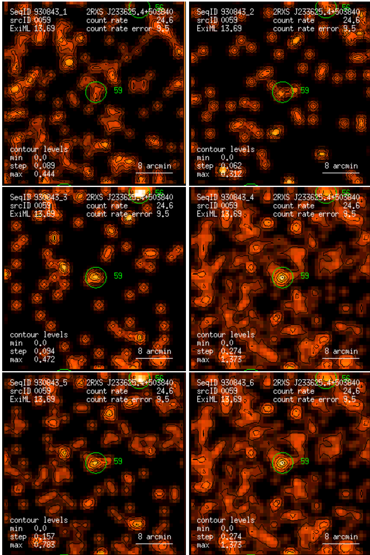
Figure 59: RASS 930843: detection 0059: band rate images, Gaussian filter: (1) PSPC channels 11 – 41, (2) 52 – 90, (3) 91 – 201, (4) 11 – 235, (5) 52 – 201, (6) 11 – 201. Broad band rates in counts/ks. Band rate contour levels in counts/ks/arcmin 2 .
