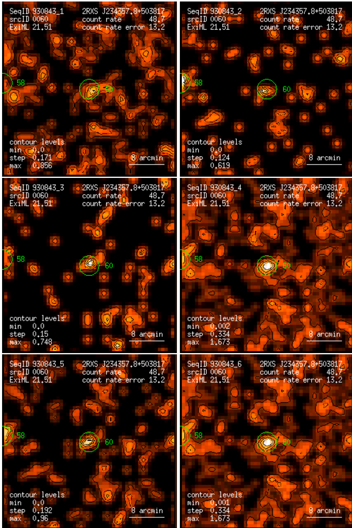
Figure 60: RASS 930843: detection 0060: band rate images, Gaussian filter: (1) PSPC channels 11 – 41, (2) 52 – 90, (3) 91 – 201, (4) 11 – 235, (5) 52 – 201, (6) 11 – 201. Broad band rates in counts/ks. Band rate contour levels in counts/ks/arcmin 2 .
