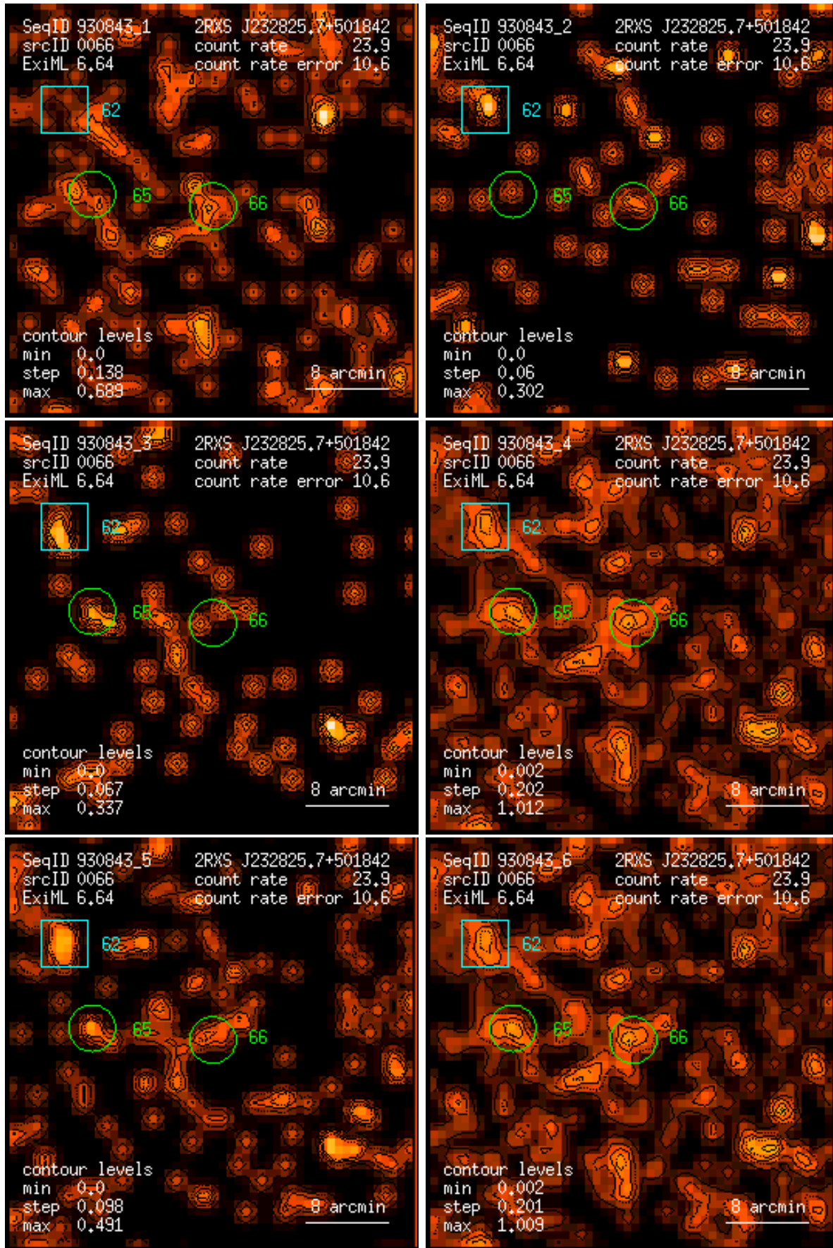
Figure 66: RASS 930843: detection 0066: band rate images, Gaussian filter: (1) PSPC channels 11 – 41, (2) 52 – 90, (3) 91 – 201, (4) 11 – 235, (5) 52 – 201, (6) 11 – 201. Broad band rates in counts/ks. Band rate contour levels in counts/ks/arcmin 2 .
