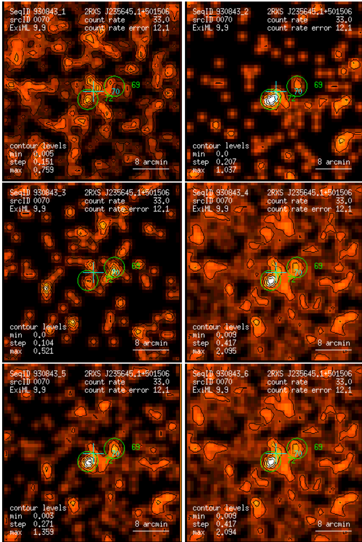
Figure 70: RASS 930843: detection 0070: band rate images, Gaussian filter: (1) PSPC channels 11 – 41, (2) 52 – 90, (3) 91 – 201, (4) 11 – 235, (5) 52 – 201, (6) 11 – 201. Broad band rates in counts/ks. Band rate contour levels in counts/ks/arcmin 2 .
