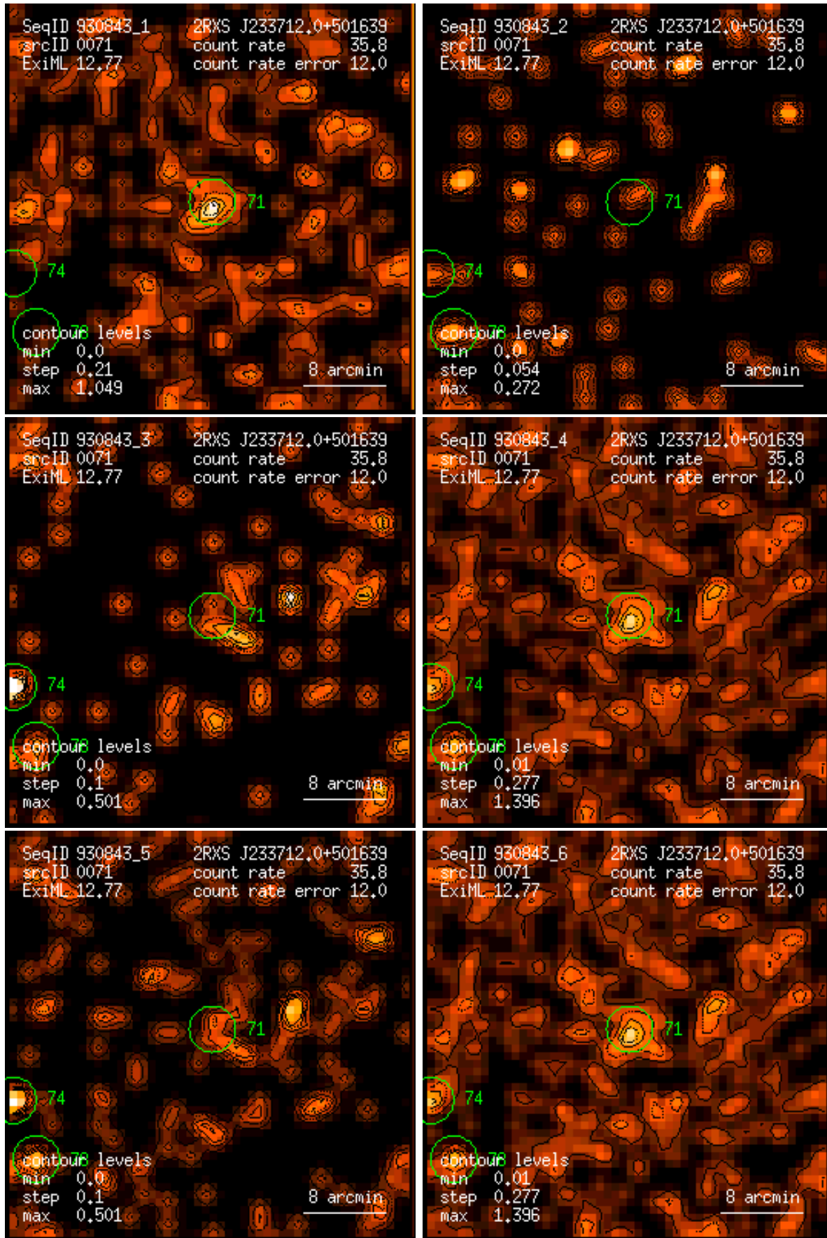
Figure 71: RASS 930843: detection 0071: band rate images, Gaussian filter: (1) PSPC channels 11 – 41, (2) 52 – 90, (3) 91 – 201, (4) 11 – 235, (5) 52 – 201, (6) 11 – 201. Broad band rates in counts/ks. Band rate contour levels in counts/ks/arcmin 2 .
