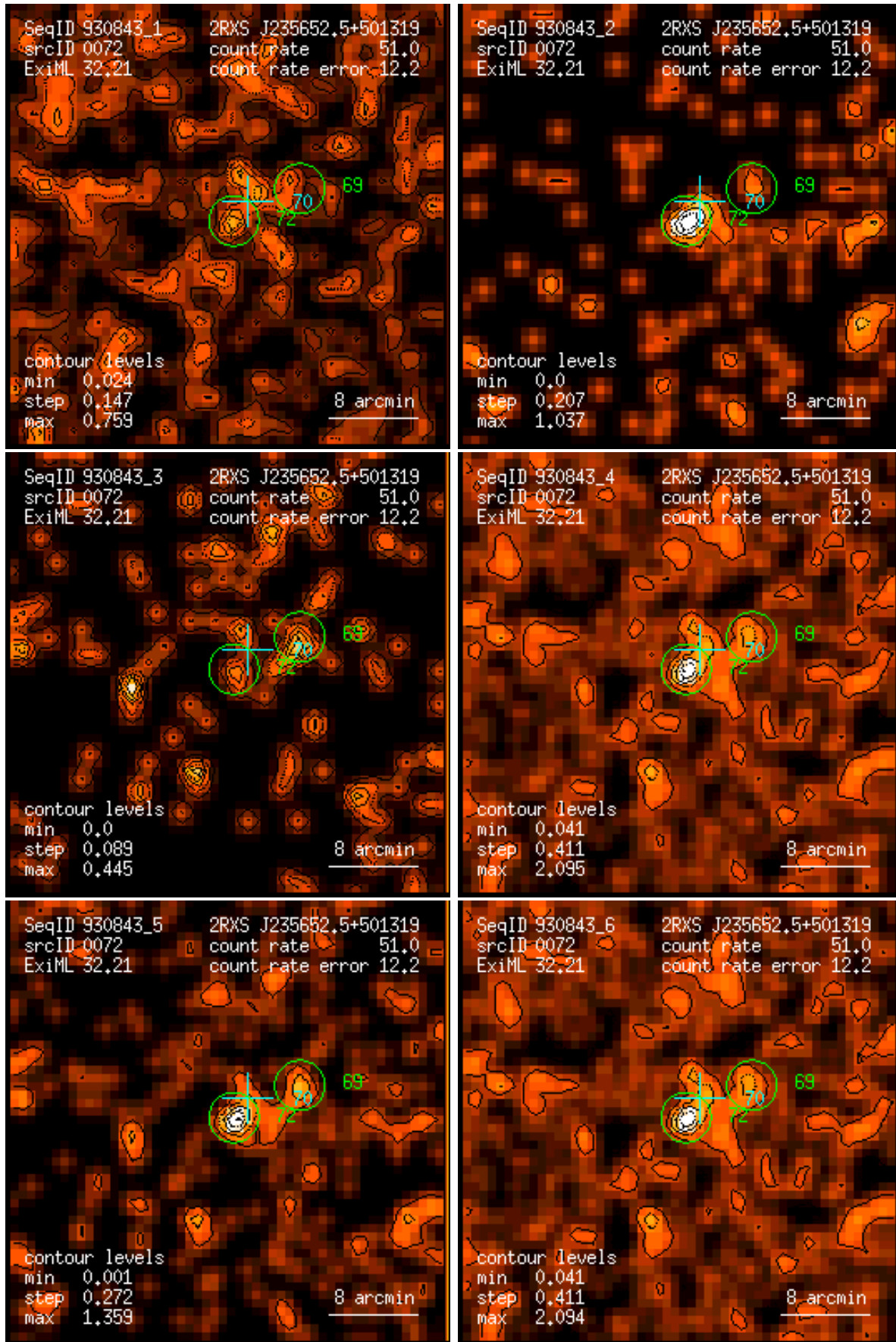
Figure 72: RASS 930843: detection 0072: band rate images, Gaussian filter: (1) PSPC channels 11 – 41, (2) 52 – 90, (3) 91 – 201, (4) 11 – 235, (5) 52 – 201, (6) 11 – 201. Broad band rates in counts/ks. Band rate contour levels in counts/ks/arcmin 2 .
