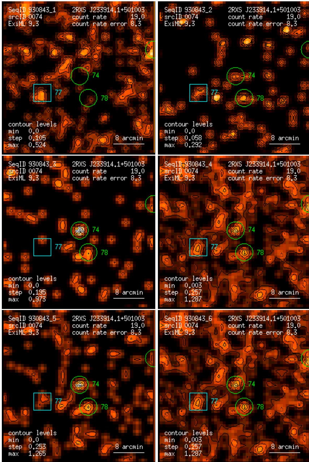
Figure 74: RASS 930843: detection 0074: band rate images, Gaussian filter: (1) PSPC channels 11 – 41, (2) 52 – 90, (3) 91 – 201, (4) 11 – 235, (5) 52 – 201, (6) 11 – 201. Broad band rates in counts/ks. Band rate contour levels in counts/ks/arcmin 2 .
