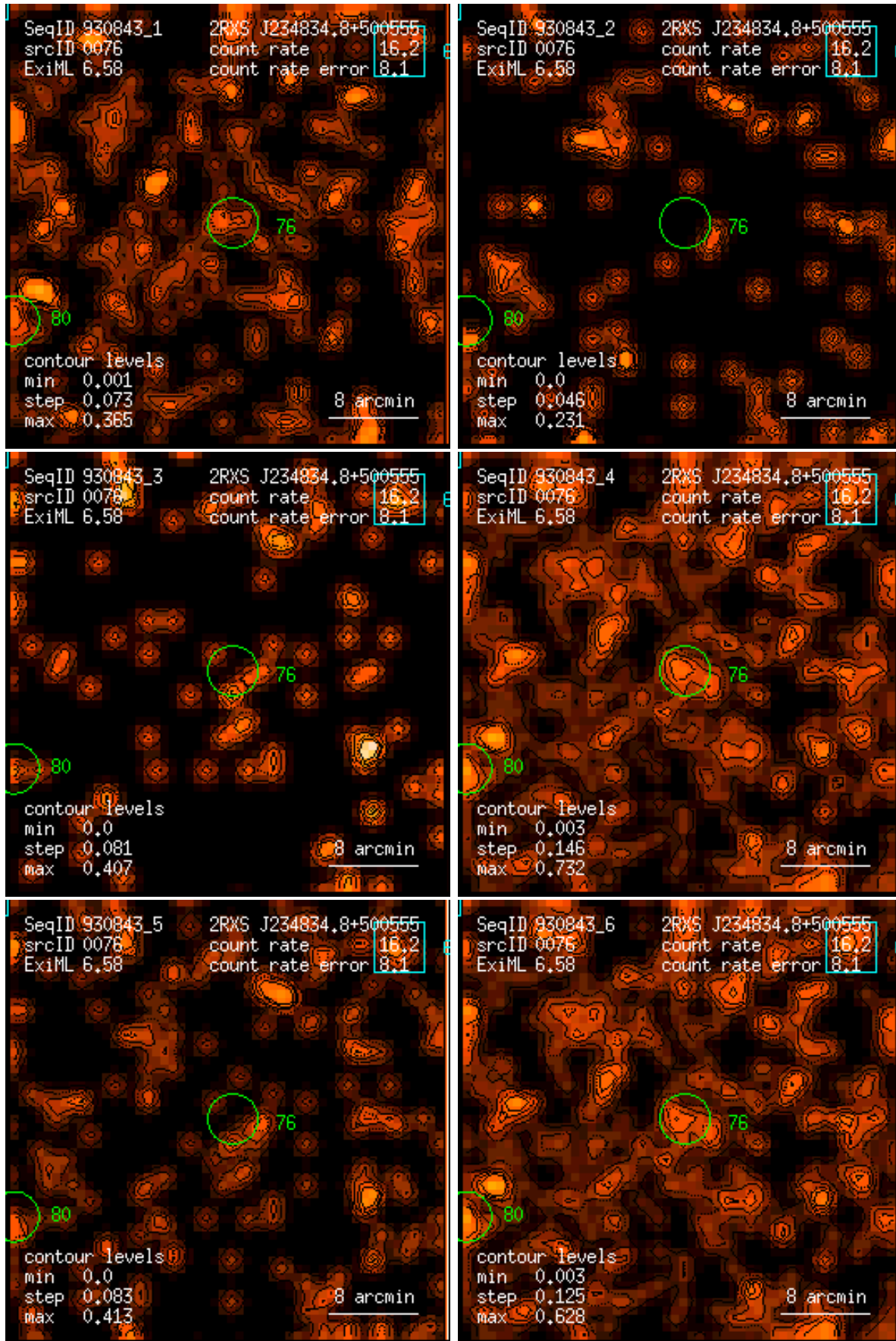
Figure 76: RASS 930843: detection 0076: band rate images, Gaussian filter: (1) PSPC channels 11 – 41, (2) 52 – 90, (3) 91 – 201, (4) 11 – 235, (5) 52 – 201, (6) 11 – 201. Broad band rates in counts/ks. Band rate contour levels in counts/ks/arcmin 2 .
