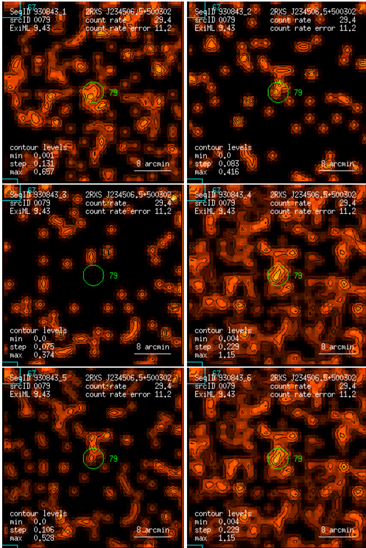
Figure 79: RASS 930843: detection 0079: band rate images, Gaussian filter: (1) PSPC channels 11 – 41, (2) 52 – 90, (3) 91 – 201, (4) 11 – 235, (5) 52 – 201, (6) 11 – 201. Broad band rates in counts/ks. Band rate contour levels in counts/ks/arcmin 2 .
