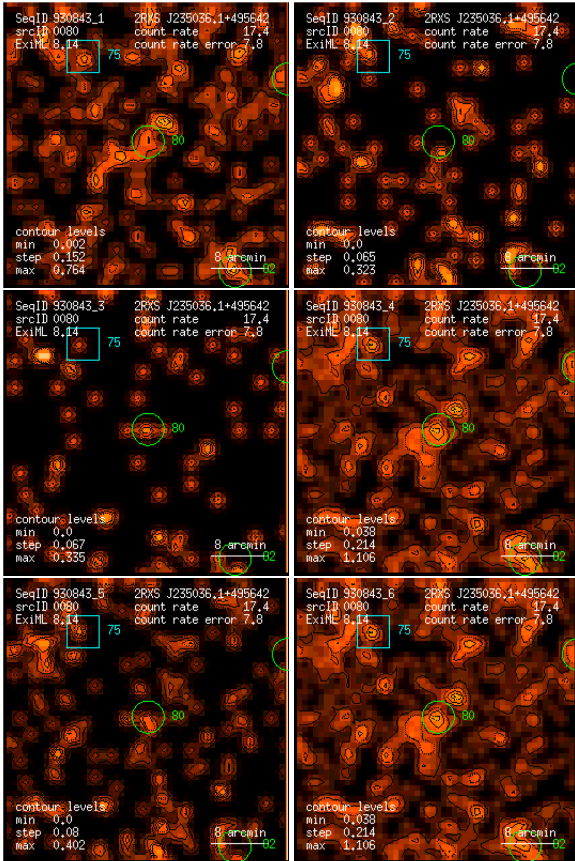
Figure 80: RASS 930843: detection 0080: band rate images, Gaussian filter: (1) PSPC channels 11 – 41, (2) 52 – 90, (3) 91 – 201, (4) 11 – 235, (5) 52 – 201, (6) 11 – 201. Broad band rates in counts/ks. Band rate contour levels in counts/ks/arcmin 2 .
