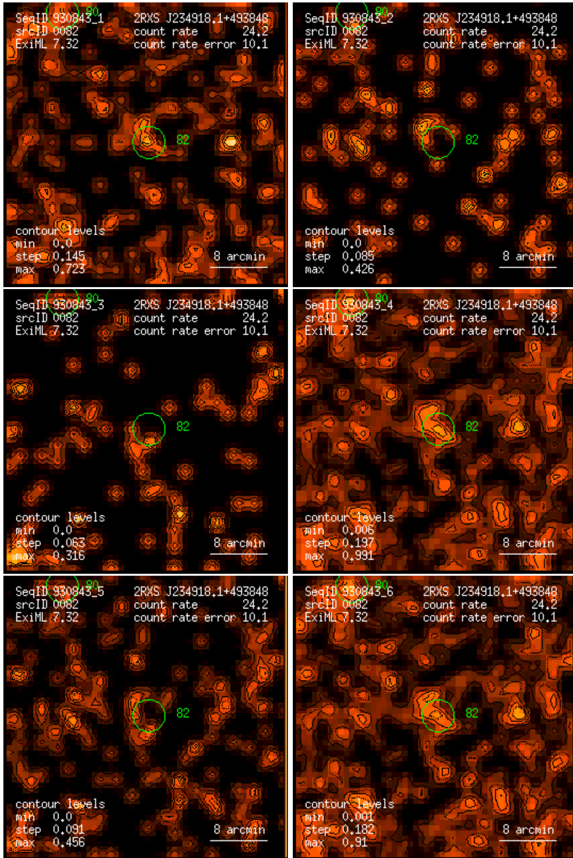
Figure 82: RASS 930843: detection 0082: band rate images, Gaussian filter: (1) PSPC channels 11 – 41, (2) 52 – 90, (3) 91 – 201, (4) 11 – 235, (5) 52 – 201, (6) 11 – 201. Broad band rates in counts/ks. Band rate contour levels in counts/ks/arcmin 2 .
