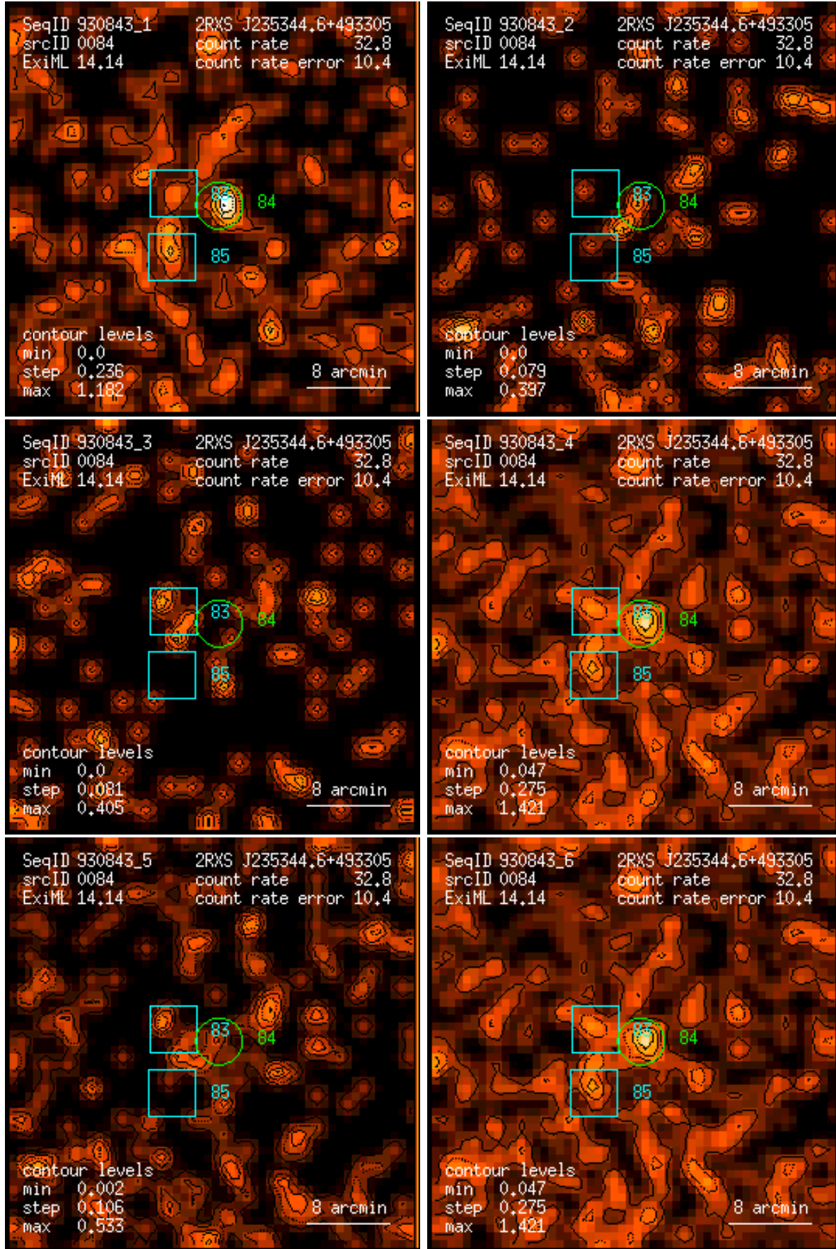
Figure 84: RASS 930843: detection 0084: band rate images, Gaussian filter: (1) PSPC channels 11 – 41, (2) 52 – 90, (3) 91 – 201, (4) 11 – 235, (5) 52 – 201, (6) 11 – 201. Broad band rates in counts/ks. Band rate contour levels in counts/ks/arcmin 2 .
