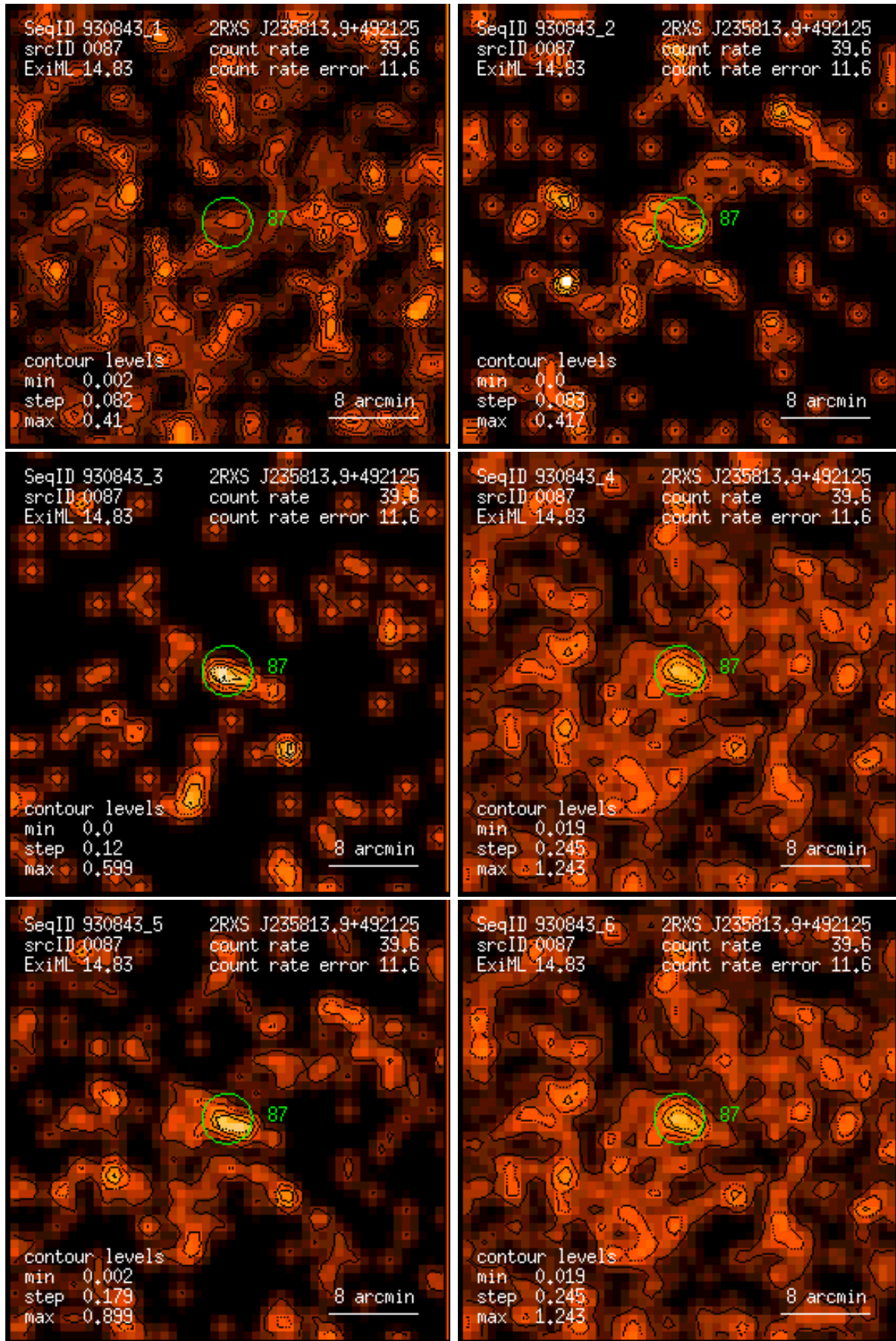
Figure 87: RASS 930843: detection 0087: band rate images, Gaussian filter: (1) PSPC channels 11 – 41, (2) 52 – 90, (3) 91 – 201, (4) 11 – 235, (5) 52 – 201, (6) 11 – 201. Broad band rates in counts/ks. Band rate contour levels in counts/ks/arcmin 2 .
