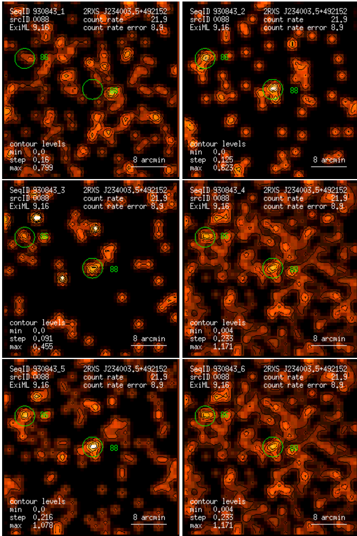
Figure 88: RASS 930843: detection 0088: band rate images, Gaussian filter: (1) PSPC channels 11 – 41, (2) 52 – 90, (3) 91 – 201, (4) 11 – 235, (5) 52 – 201, (6) 11 – 201. Broad band rates in counts/ks. Band rate contour levels in counts/ks/arcmin 2 .
