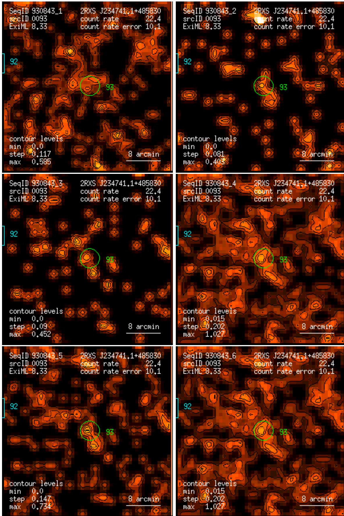
Figure 93: RASS 930843: detection 0093: band rate images, Gaussian filter: (1) PSPC channels 11 – 41, (2) 52 – 90, (3) 91 – 201, (4) 11 – 235, (5) 52 – 201, (6) 11 – 201. Broad band rates in counts/ks. Band rate contour levels in counts/ks/arcmin 2 .
