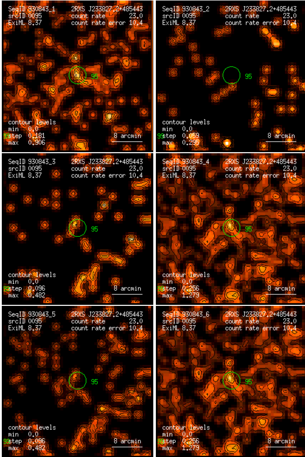
Figure 95: RASS 930843: detection 0095: band rate images, Gaussian filter: (1) PSPC channels 11 – 41, (2) 52 – 90, (3) 91 – 201, (4) 11 – 235, (5) 52 – 201, (6) 11 – 201. Broad band rates in counts/ks. Band rate contour levels in counts/ks/arcmin 2 .
