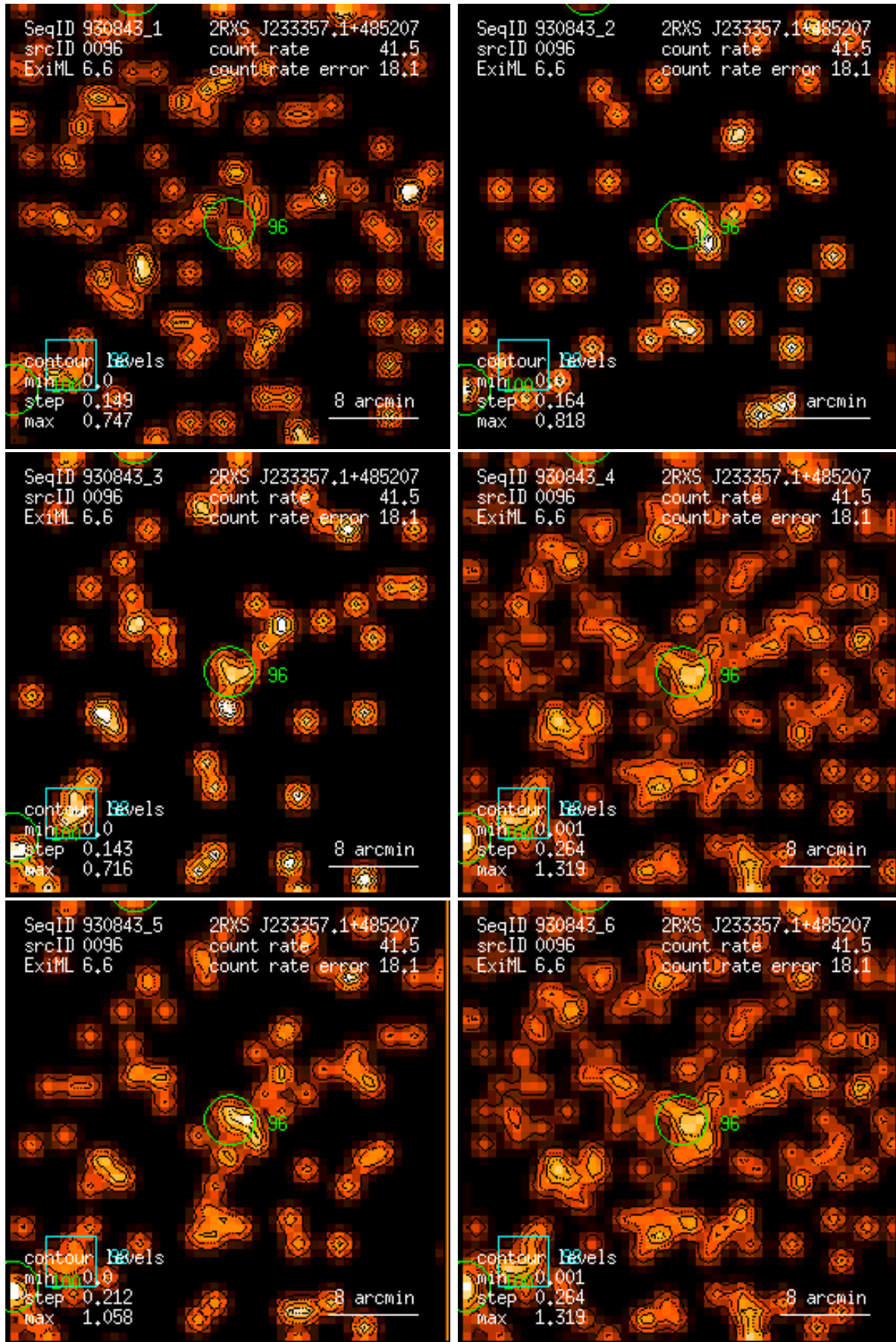
Figure 96: RASS 930843: detection 0096: band rate images, Gaussian filter: (1) PSPC channels 11 – 41, (2) 52 – 90, (3) 91 – 201, (4) 11 – 235, (5) 52 – 201, (6) 11 – 201. Broad band rates in counts/ks. Band rate contour levels in counts/ks/arcmin 2 .
