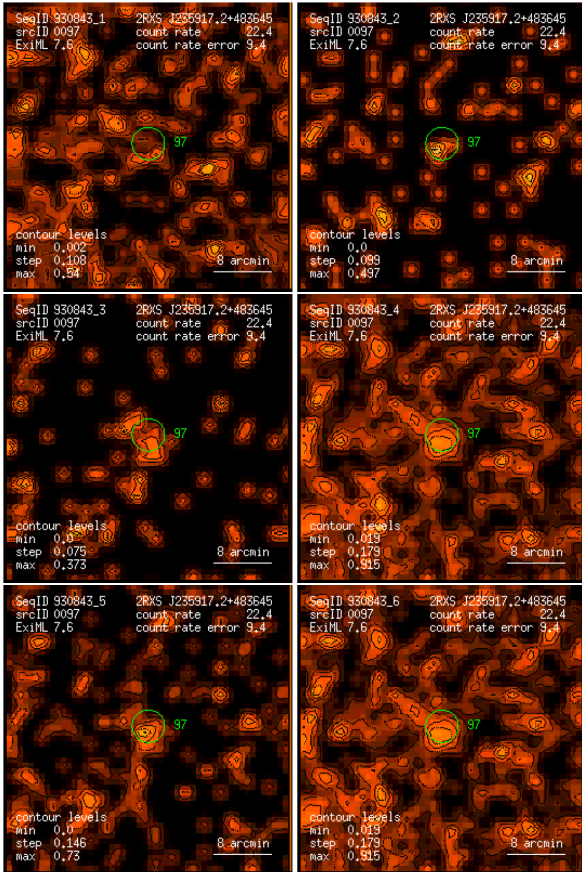
Figure 97: RASS 930843: detection 0097: band rate images, Gaussian filter: (1) PSPC channels 11 – 41, (2) 52 – 90, (3) 91 – 201, (4) 11 – 235, (5) 52 – 201, (6) 11 – 201. Broad band rates in counts/ks. Band rate contour levels in counts/ks/arcmin 2 .
