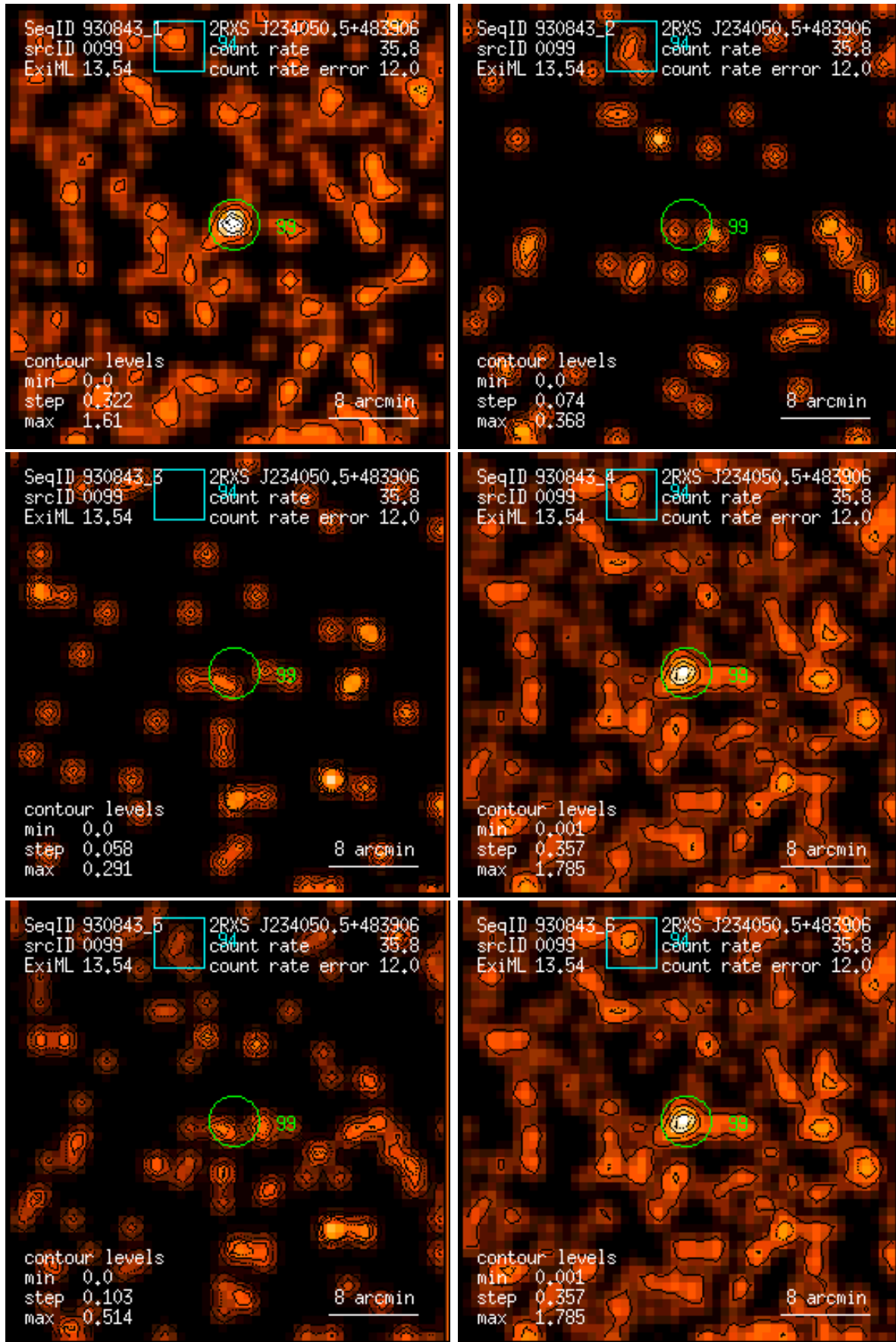
Figure 99: RASS 930843: detection 0099: band rate images, Gaussian filter: (1) PSPC channels 11 – 41, (2) 52 – 90, (3) 91 – 201, (4) 11 – 235, (5) 52 – 201, (6) 11 – 201. Broad band rates in counts/ks. Band rate contour levels in counts/ks/arcmin 2 .
