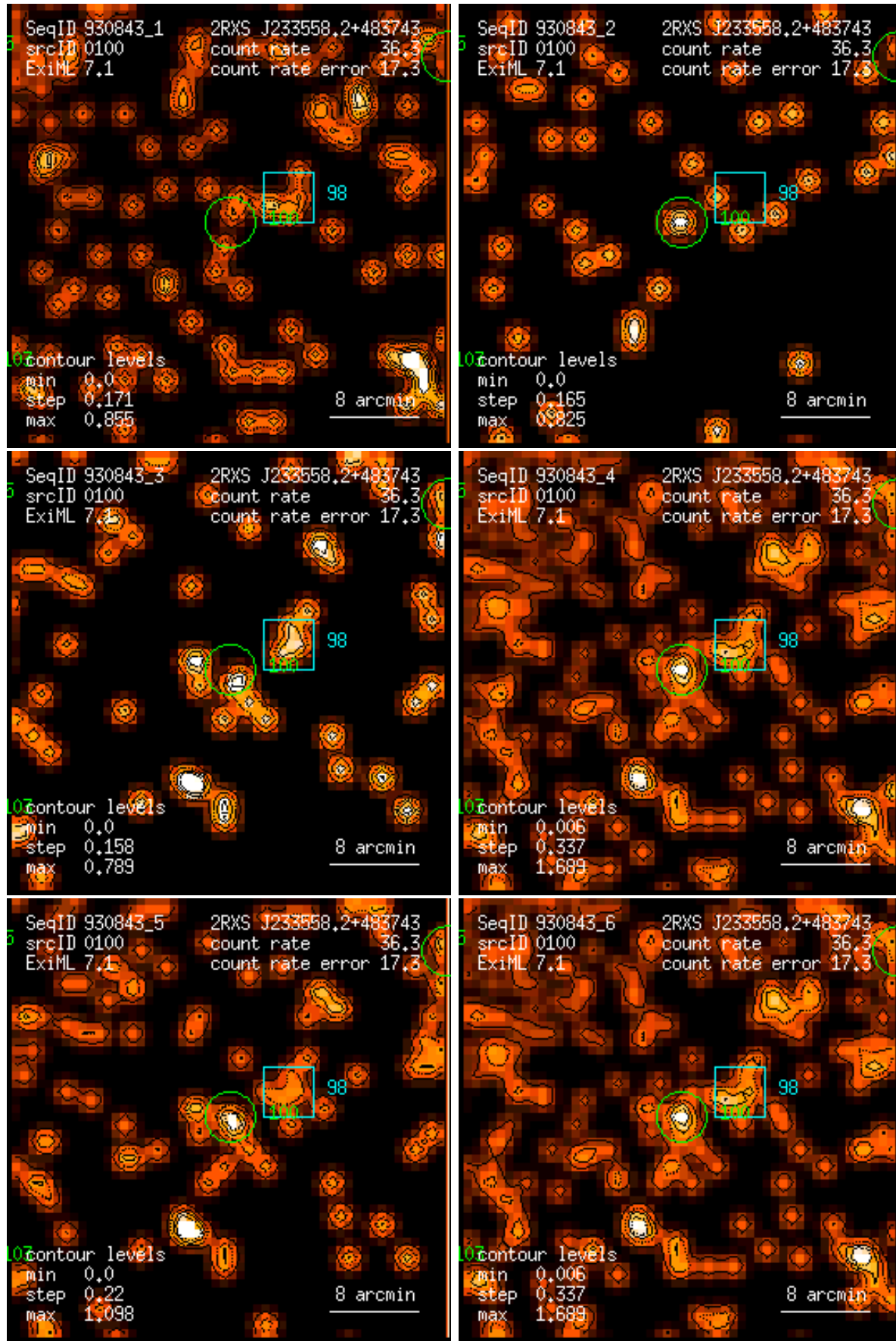
Figure 100: RASS 930843: detection 0100: band rate images, Gaussian filter: (1) PSPC channels 11 – 41, (2) 52 – 90, (3) 91 – 201, (4) 11 – 235, (5) 52 – 201, (6) 11 – 201. Broad band rates in counts/ks. Band rate contour levels in counts/ks/arcmin 2 .
