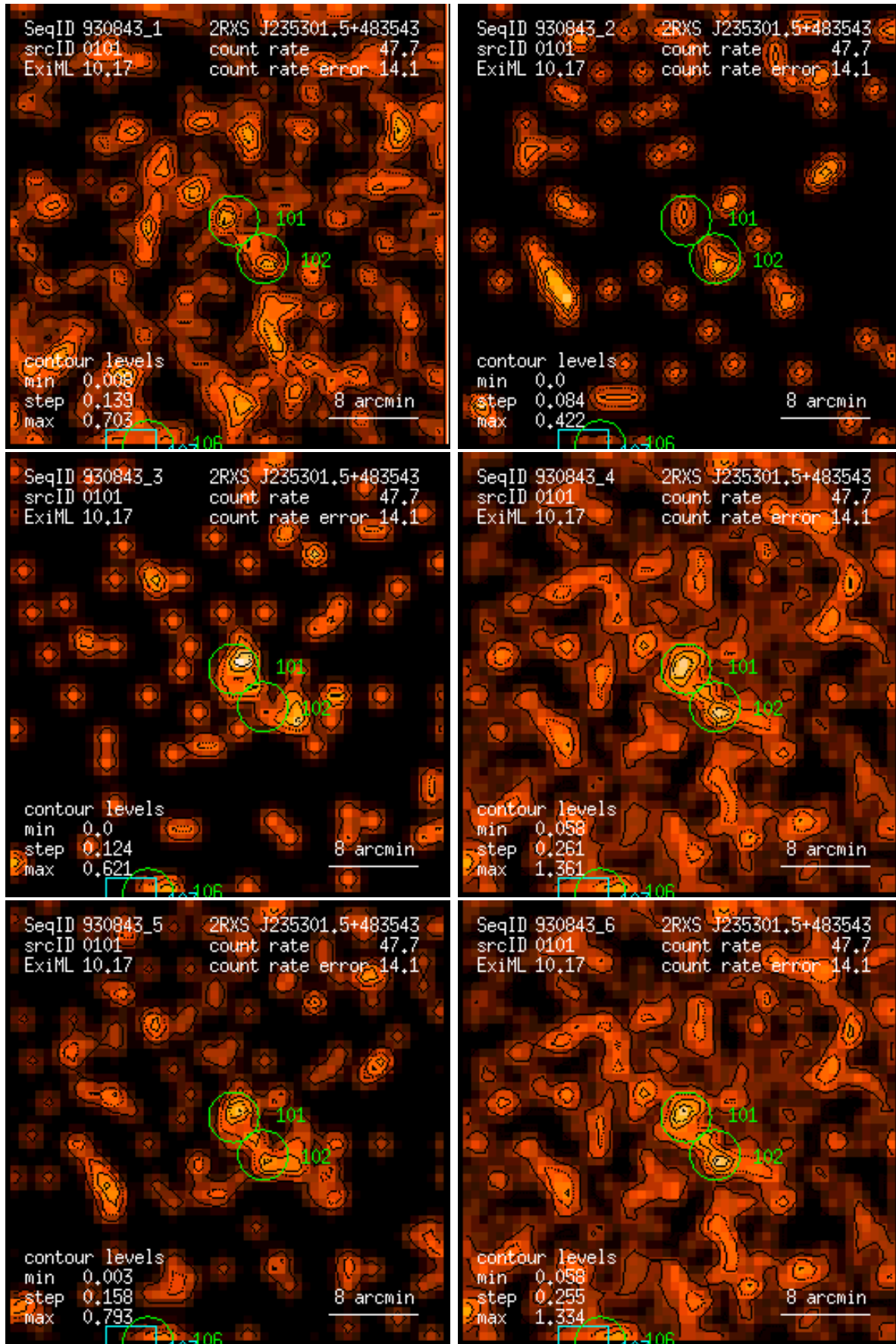
Figure 101: RASS 930843: detection 0101: band rate images, Gaussian filter: (1) PSPC channels 11 – 41, (2) 52 – 90, (3) 91 – 201, (4) 11 – 235, (5) 52 – 201, (6) 11 – 201. Broad band rates in counts/ks. Band rate contour levels in counts/ks/arcmin 2 .
