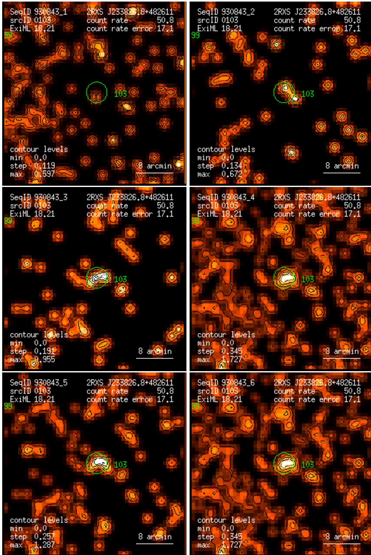
Figure 103: RASS 930843: detection 0103: band rate images, Gaussian filter: (1) PSPC channels 11 – 41, (2) 52 – 90, (3) 91 – 201, (4) 11 – 235, (5) 52 – 201, (6) 11 – 201. Broad band rates in counts/ks. Band rate contour levels in counts/ks/arcmin 2 .
