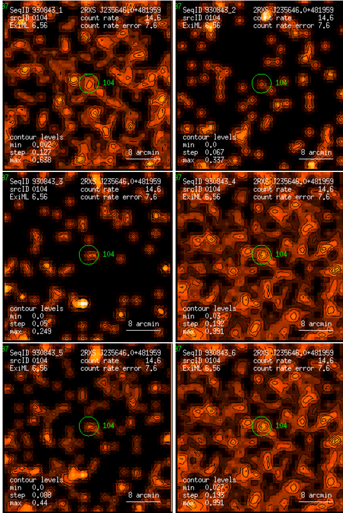
Figure 104: RASS 930843: detection 0104: band rate images, Gaussian filter: (1) PSPC channels 11 – 41, (2) 52 – 90, (3) 91 – 201, (4) 11 – 235, (5) 52 – 201, (6) 11 – 201. Broad band rates in counts/ks. Band rate contour levels in counts/ks/arcmin 2 .
