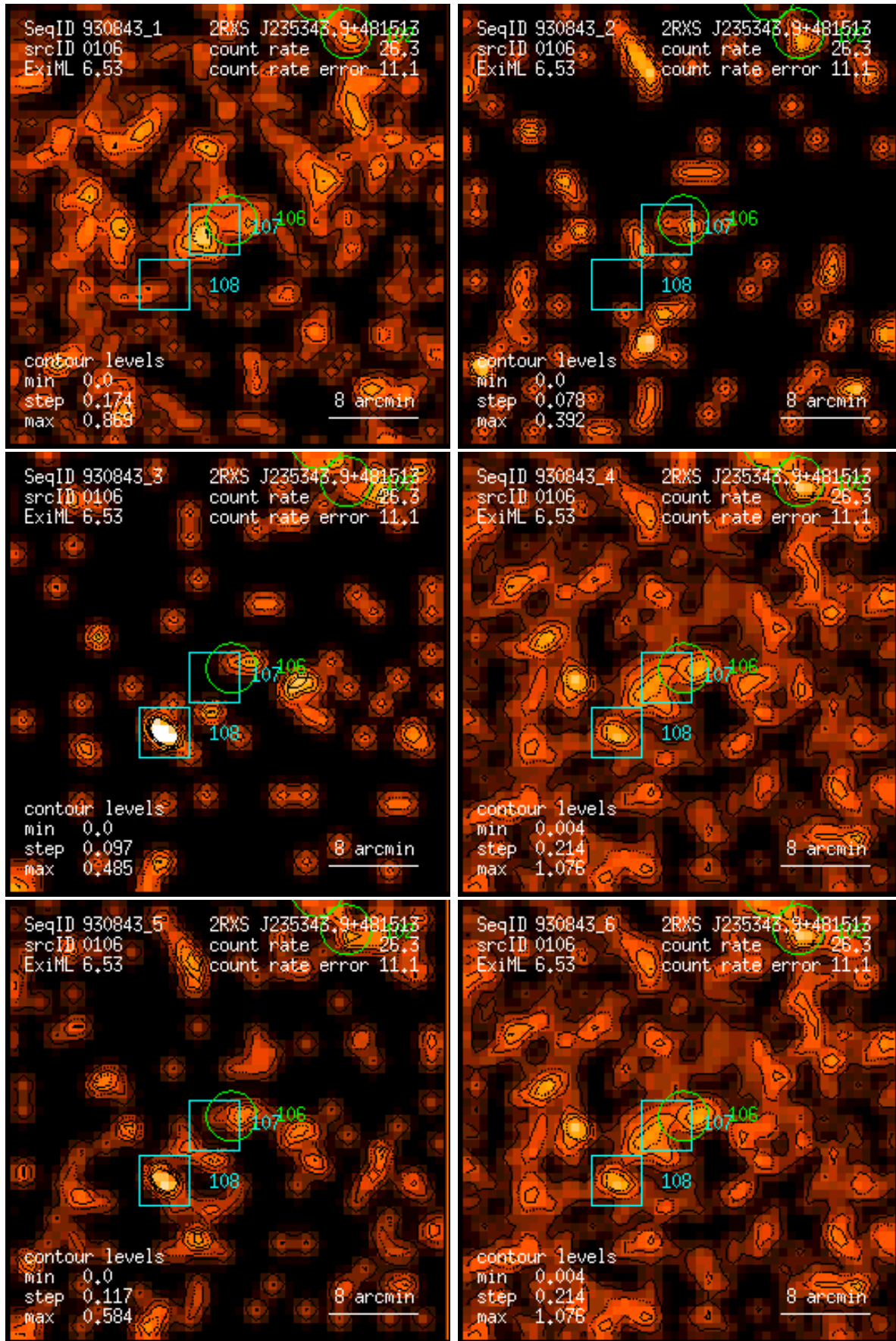
Figure 106: RASS 930843: detection 0106: band rate images, Gaussian filter: (1) PSPC channels 11 – 41, (2) 52 – 90, (3) 91 – 201, (4) 11 – 235, (5) 52 – 201, (6) 11 – 201. Broad band rates in counts/ks. Band rate contour levels in counts/ks/arcmin 2 .
